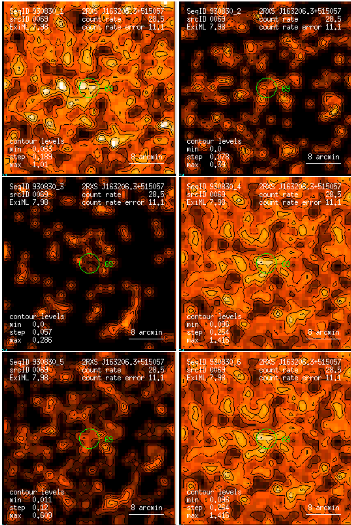
Figure 69: RASS 930830: detection 0069: band rate images, Gaussian filter: (1) PSPC channels 11 – 41, (2) 52 – 90, (3) 91 – 201, (4) 11 – 235, (5) 52 – 201, (6) 11 – 201. Broad band rates in counts/ks. Band rate contour levels in counts/ks/arcmin 2 .
