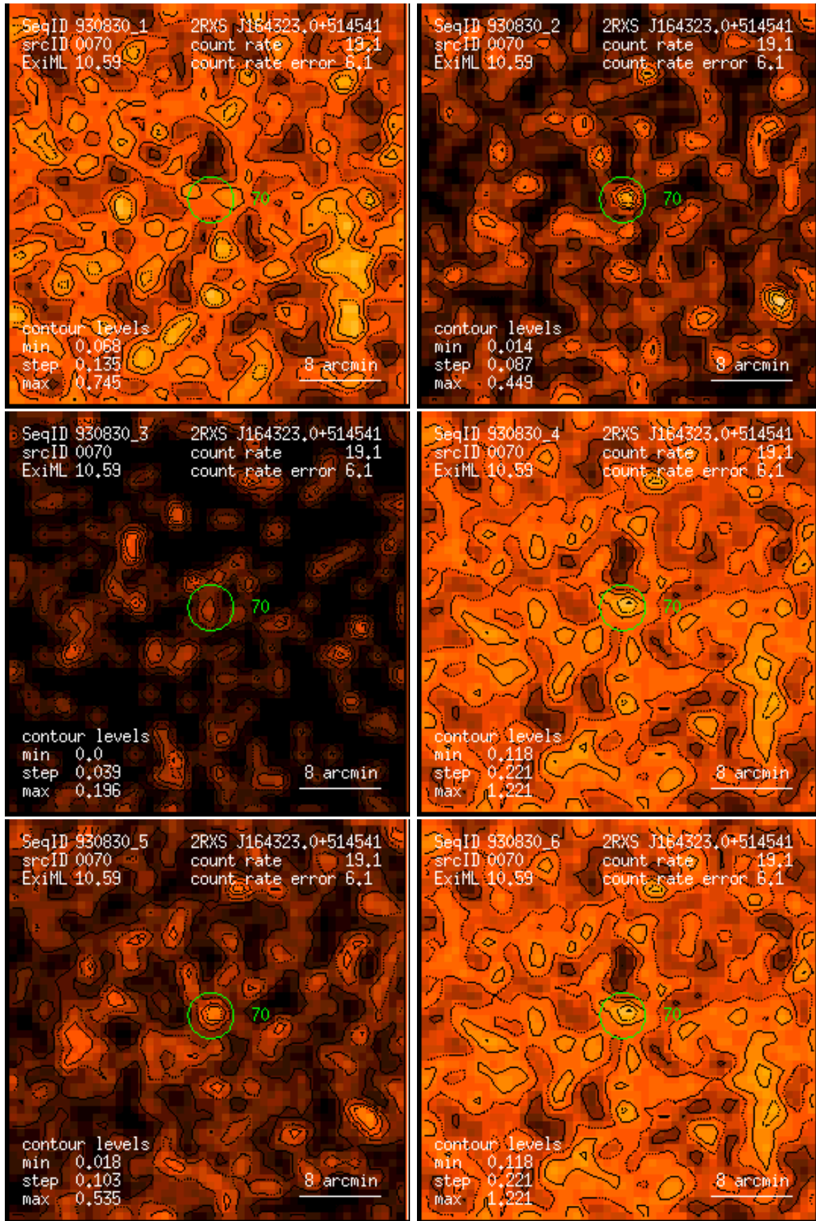
Figure 70: RASS 930830: detection 0070: band rate images, Gaussian filter: (1) PSPC channels 11 – 41, (2) 52 – 90, (3) 91 – 201, (4) 11 – 235, (5) 52 – 201, (6) 11 – 201. Broad band rates in counts/ks. Band rate contour levels in counts/ks/arcmin 2 .
