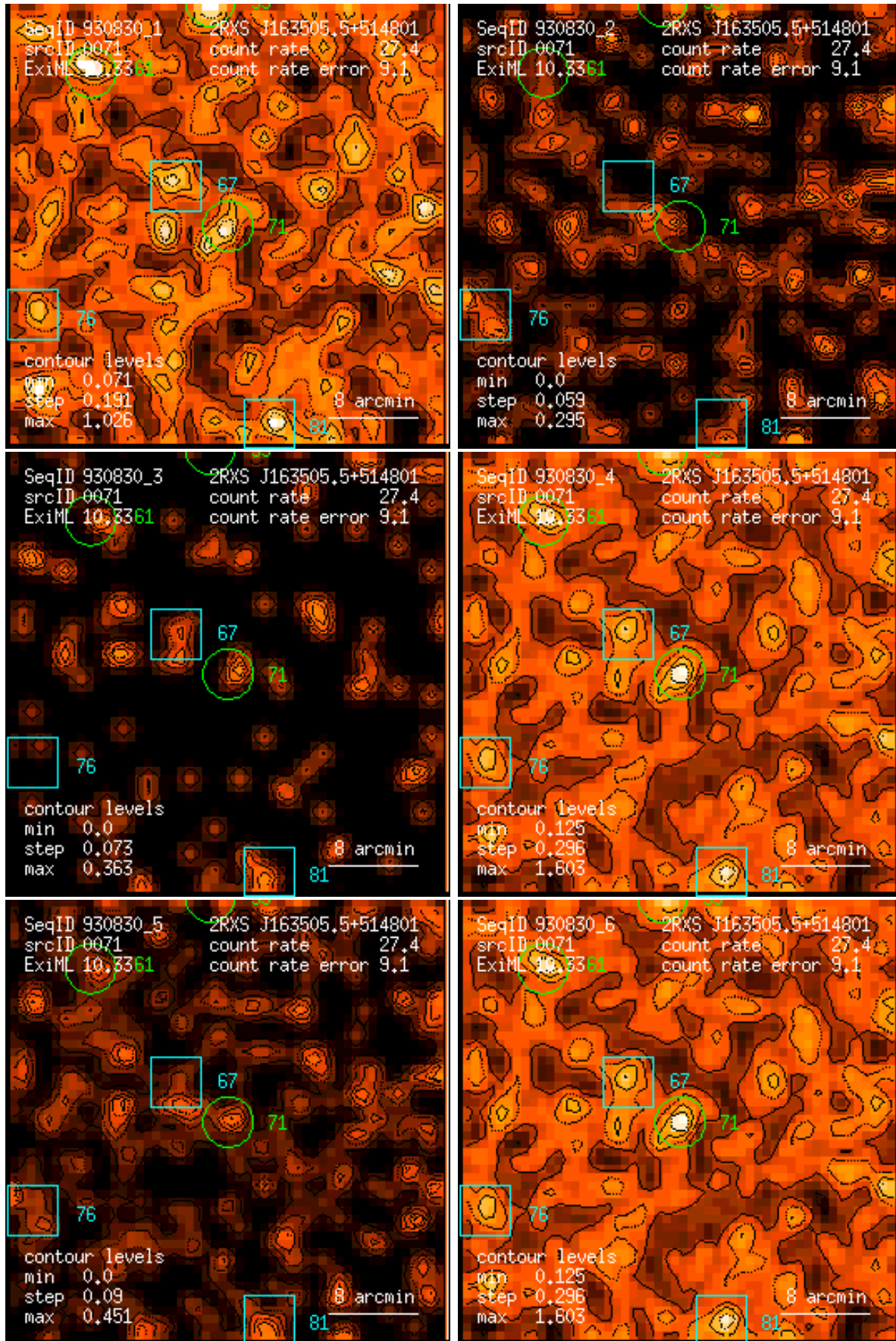
Figure 71: RASS 930830: detection 0071: band rate images, Gaussian filter: (1) PSPC channels 11 – 41, (2) 52 – 90, (3) 91 – 201, (4) 11 – 235, (5) 52 – 201, (6) 11 – 201. Broad band rates in counts/ks. Band rate contour levels in counts/ks/arcmin 2 .
