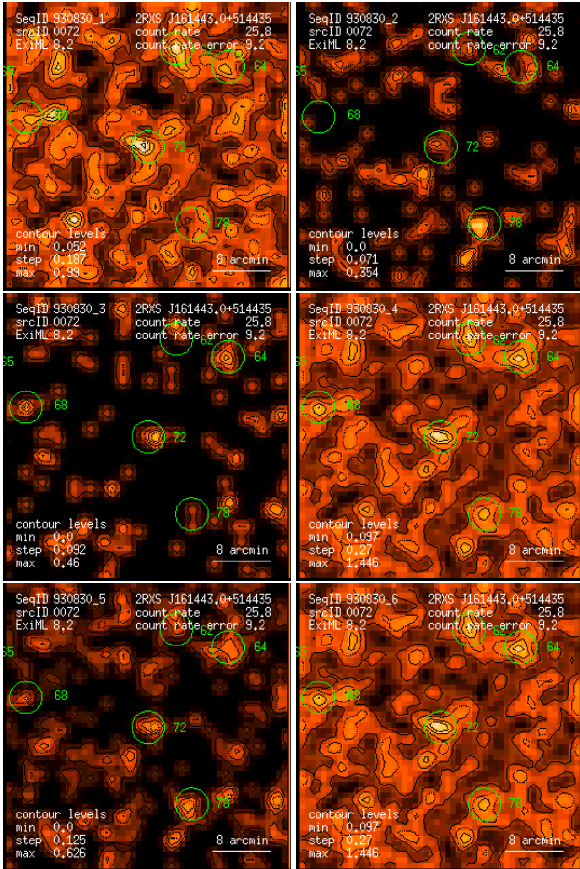
Figure 72: RASS 930830: detection 0072: band rate images, Gaussian filter: (1) PSPC channels 11 – 41, (2) 52 – 90, (3) 91 – 201, (4) 11 – 235, (5) 52 – 201, (6) 11 – 201. Broad band rates in counts/ks. Band rate contour levels in counts/ks/arcmin 2 .
