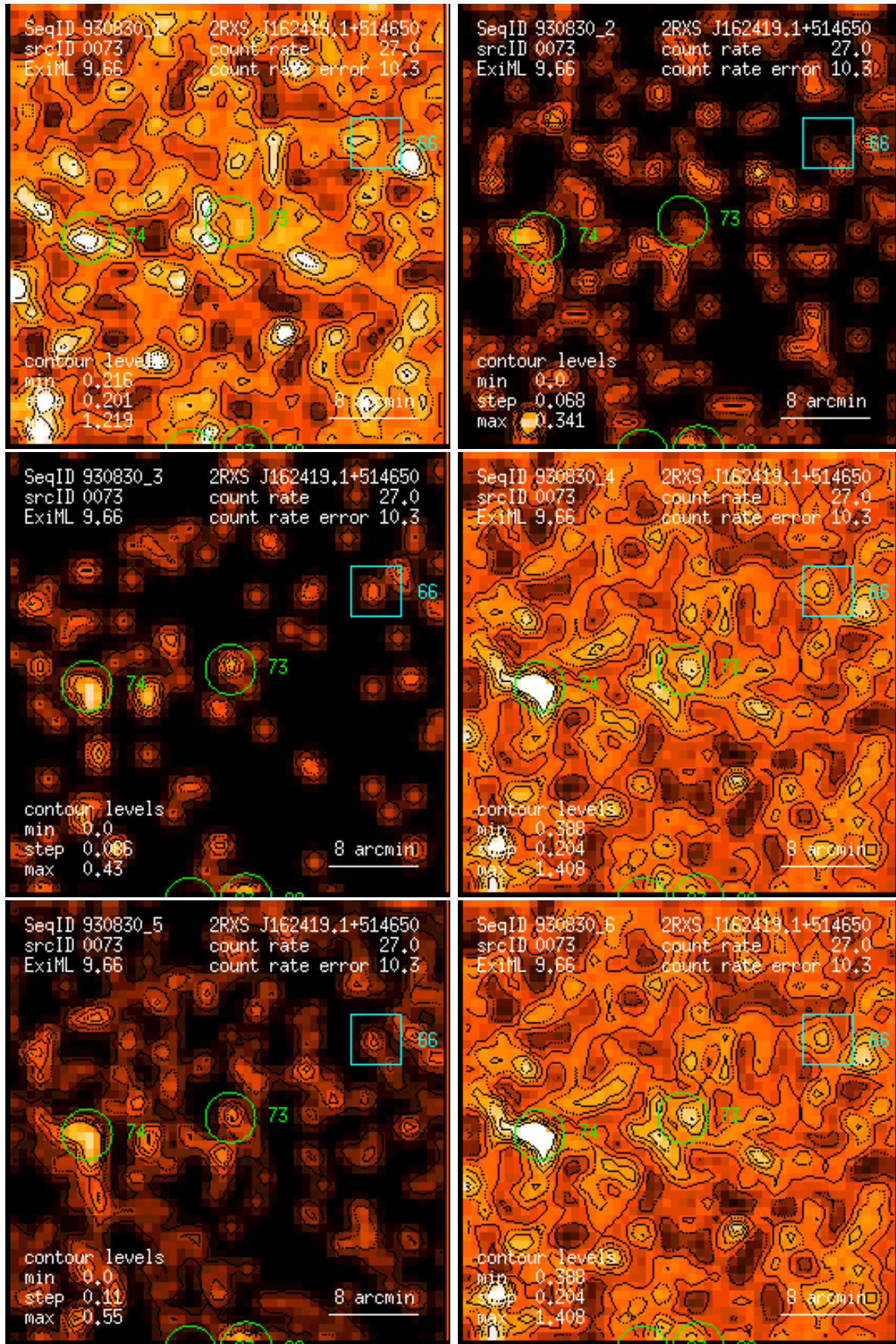
Figure 73: RASS 930830: detection 0073: band rate images, Gaussian filter: (1) PSPC channels 11 – 41, (2) 52 – 90, (3) 91 – 201, (4) 11 – 235, (5) 52 – 201, (6) 11 – 201. Broad band rates in counts/ks. Band rate contour levels in counts/ks/arcmin 2 .
