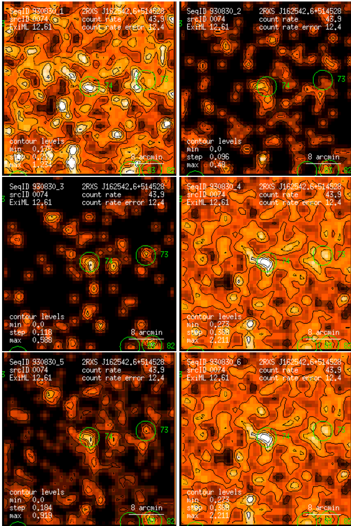
Figure 74: RASS 930830: detection 0074: band rate images, Gaussian filter: (1) PSPC channels 11 – 41, (2) 52 – 90, (3) 91 – 201, (4) 11 – 235, (5) 52 – 201, (6) 11 – 201. Broad band rates in counts/ks. Band rate contour levels in counts/ks/arcmin 2 .
