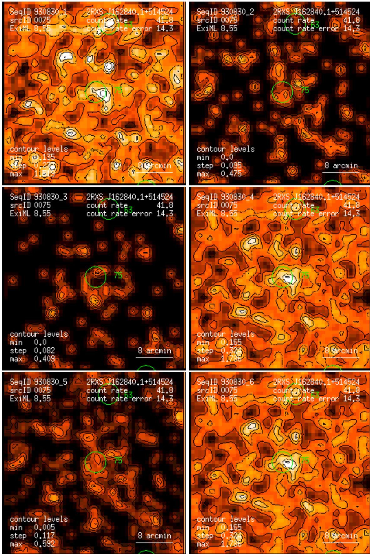
Figure 75: RASS 930830: detection 0075: band rate images, Gaussian filter: (1) PSPC channels 11 – 41, (2) 52 – 90, (3) 91 – 201, (4) 11 – 235, (5) 52 – 201, (6) 11 – 201. Broad band rates in counts/ks. Band rate contour levels in counts/ks/arcmin 2 .
