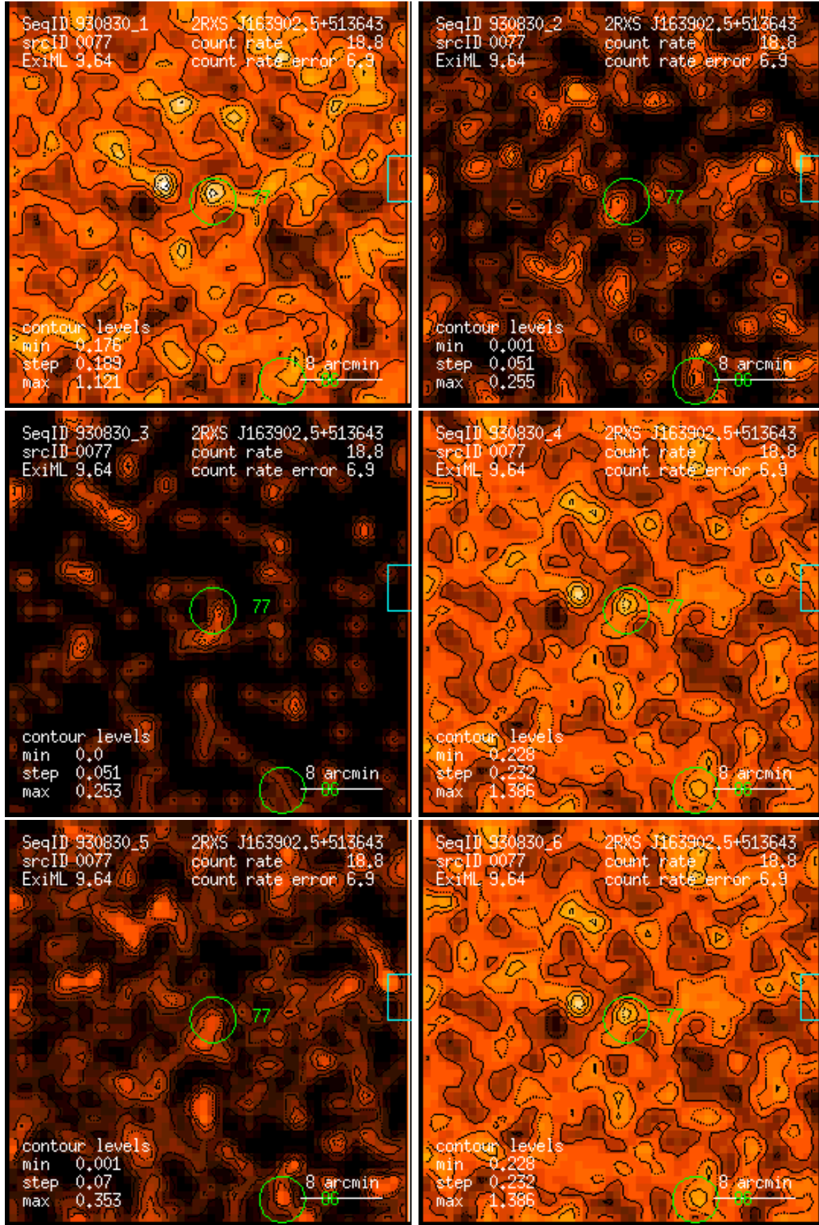
Figure 77: RASS 930830: detection 0077: band rate images, Gaussian filter: (1) PSPC channels 11 – 41, (2) 52 – 90, (3) 91 – 201, (4) 11 – 235, (5) 52 – 201, (6) 11 – 201. Broad band rates in counts/ks. Band rate contour levels in counts/ks/arcmin 2 .
