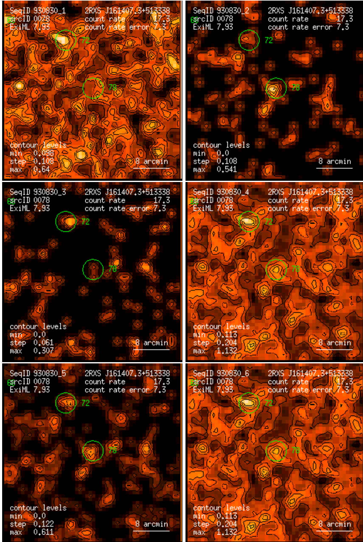
Figure 78: RASS 930830: detection 0078: band rate images, Gaussian filter: (1) PSPC channels 11 – 41, (2) 52 – 90, (3) 91 – 201, (4) 11 – 235, (5) 52 – 201, (6) 11 – 201. Broad band rates in counts/ks. Band rate contour levels in counts/ks/arcmin 2 .
