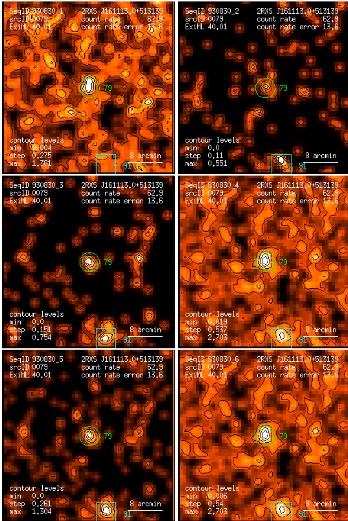
Figure 79: RASS 930830: detection 0079: band rate images, Gaussian filter: (1) PSPC channels 11 – 41, (2) 52 – 90, (3) 91 – 201, (4) 11 – 235, (5) 52 – 201, (6) 11 – 201. Broad band rates in counts/ks. Band rate contour levels in counts/ks/arcmin 2 .
