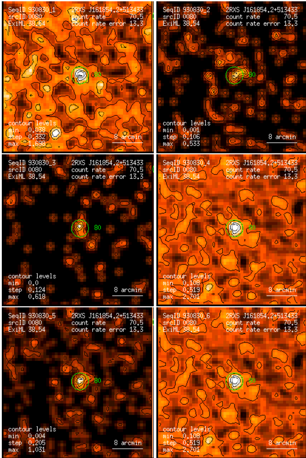
Figure 80: RASS 930830: detection 0080: band rate images, Gaussian filter: (1) PSPC channels 11 – 41, (2) 52 – 90, (3) 91 – 201, (4) 11 – 235, (5) 52 – 201, (6) 11 – 201. Broad band rates in counts/ks. Band rate contour levels in counts/ks/arcmin 2 .
