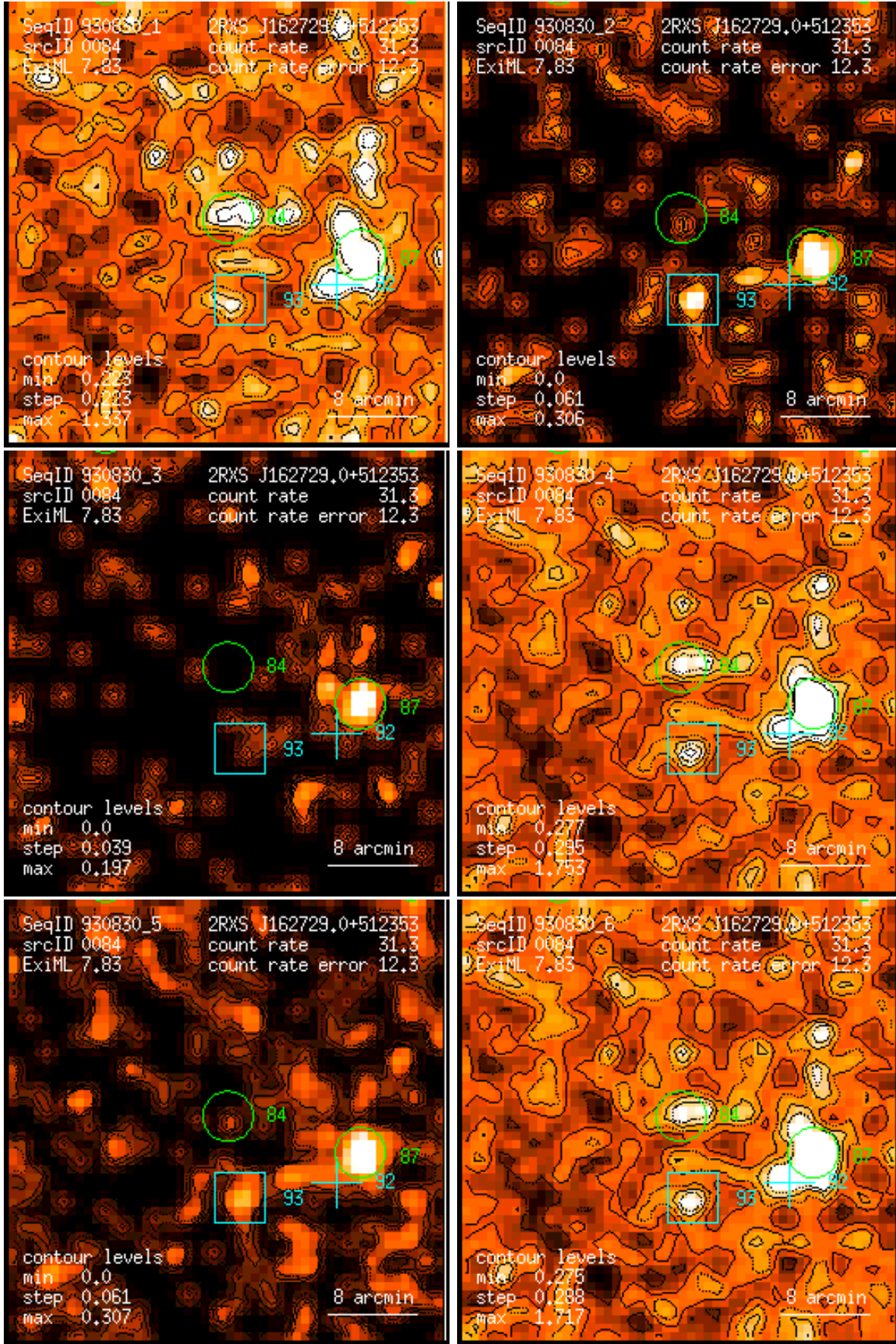
Figure 84: RASS 930830: detection 0084: band rate images, Gaussian filter: (1) PSPC channels 11 – 41, (2) 52 – 90, (3) 91 – 201, (4) 11 – 235, (5) 52 – 201, (6) 11 – 201. Broad band rates in counts/ks. Band rate contour levels in counts/ks/arcmin 2 .
