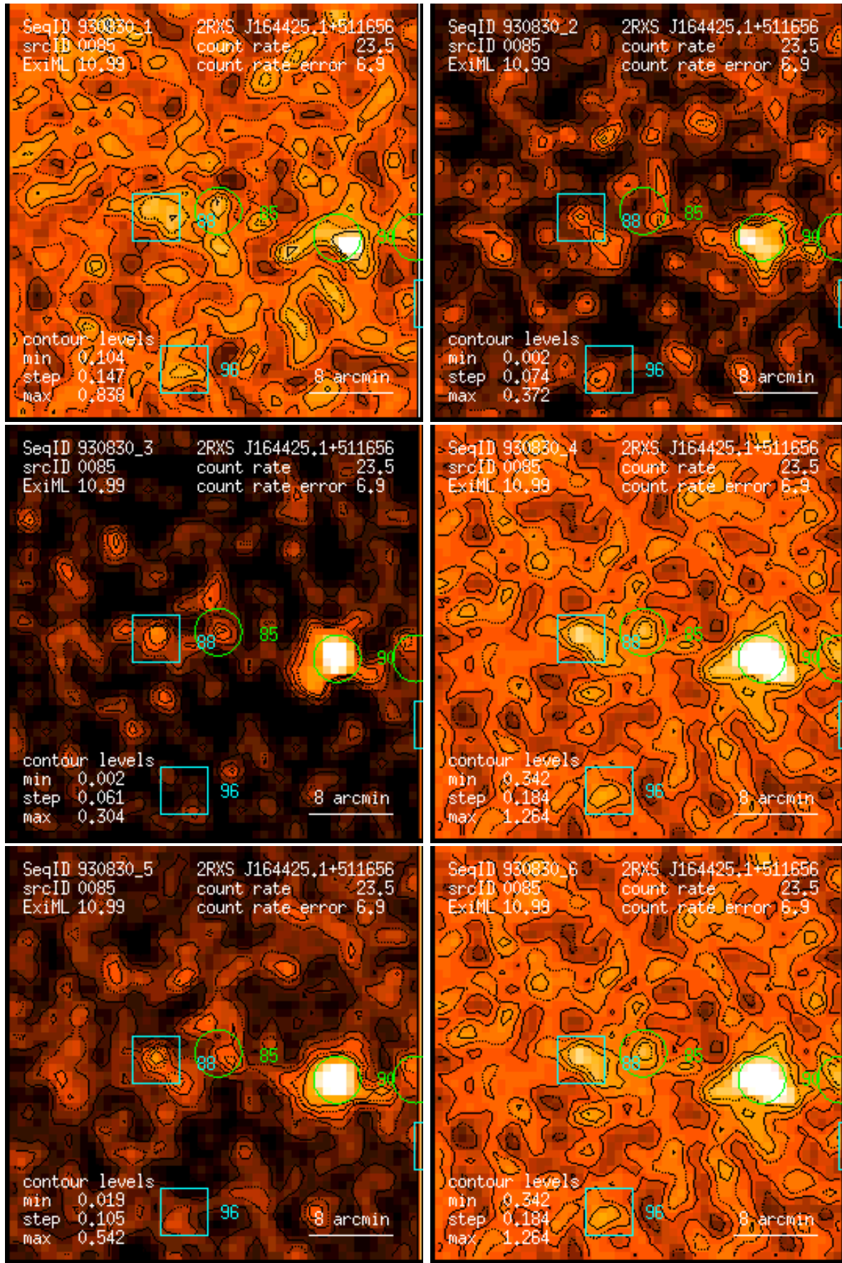
Figure 85: RASS 930830: detection 0085: band rate images, Gaussian filter: (1) PSPC channels 11 – 41, (2) 52 – 90, (3) 91 – 201, (4) 11 – 235, (5) 52 – 201, (6) 11 – 201. Broad band rates in counts/ks. Band rate contour levels in counts/ks/arcmin 2 .
