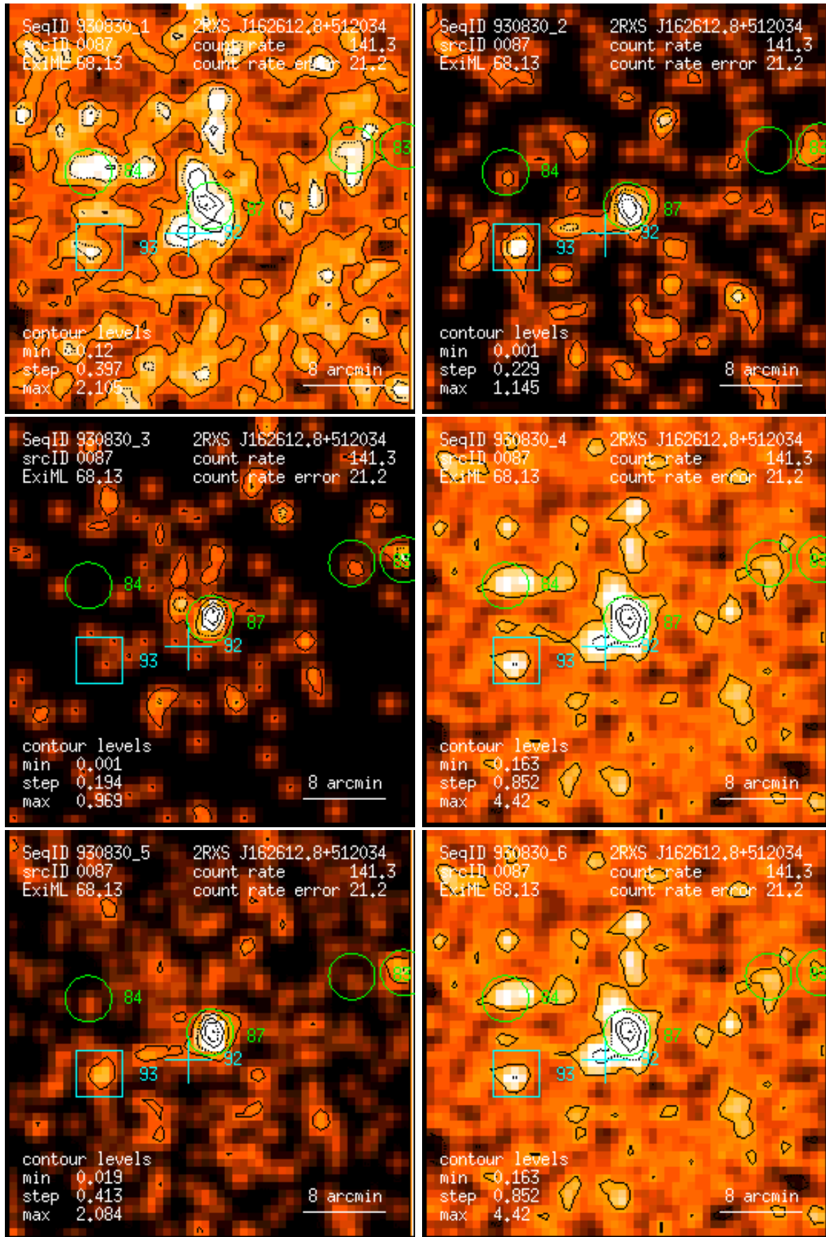
Figure 87: RASS 930830: detection 0087: band rate images, Gaussian filter: (1) PSPC channels 11 – 41, (2) 52 – 90, (3) 91 – 201, (4) 11 – 235, (5) 52 – 201, (6) 11 – 201. Broad band rates in counts/ks. Band rate contour levels in counts/ks/arcmin 2 .
