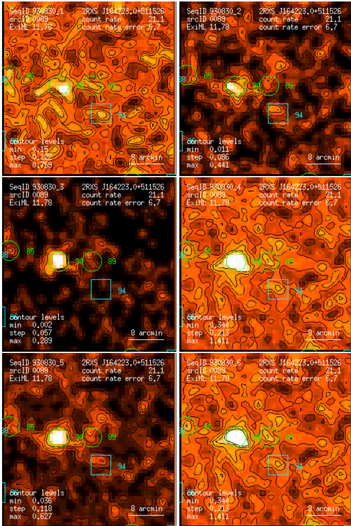
Figure 89: RASS 930830: detection 0089: band rate images, Gaussian filter: (1) PSPC channels 11 – 41, (2) 52 – 90, (3) 91 – 201, (4) 11 – 235, (5) 52 – 201, (6) 11 – 201. Broad band rates in counts/ks. Band rate contour levels in counts/ks/arcmin 2 .
