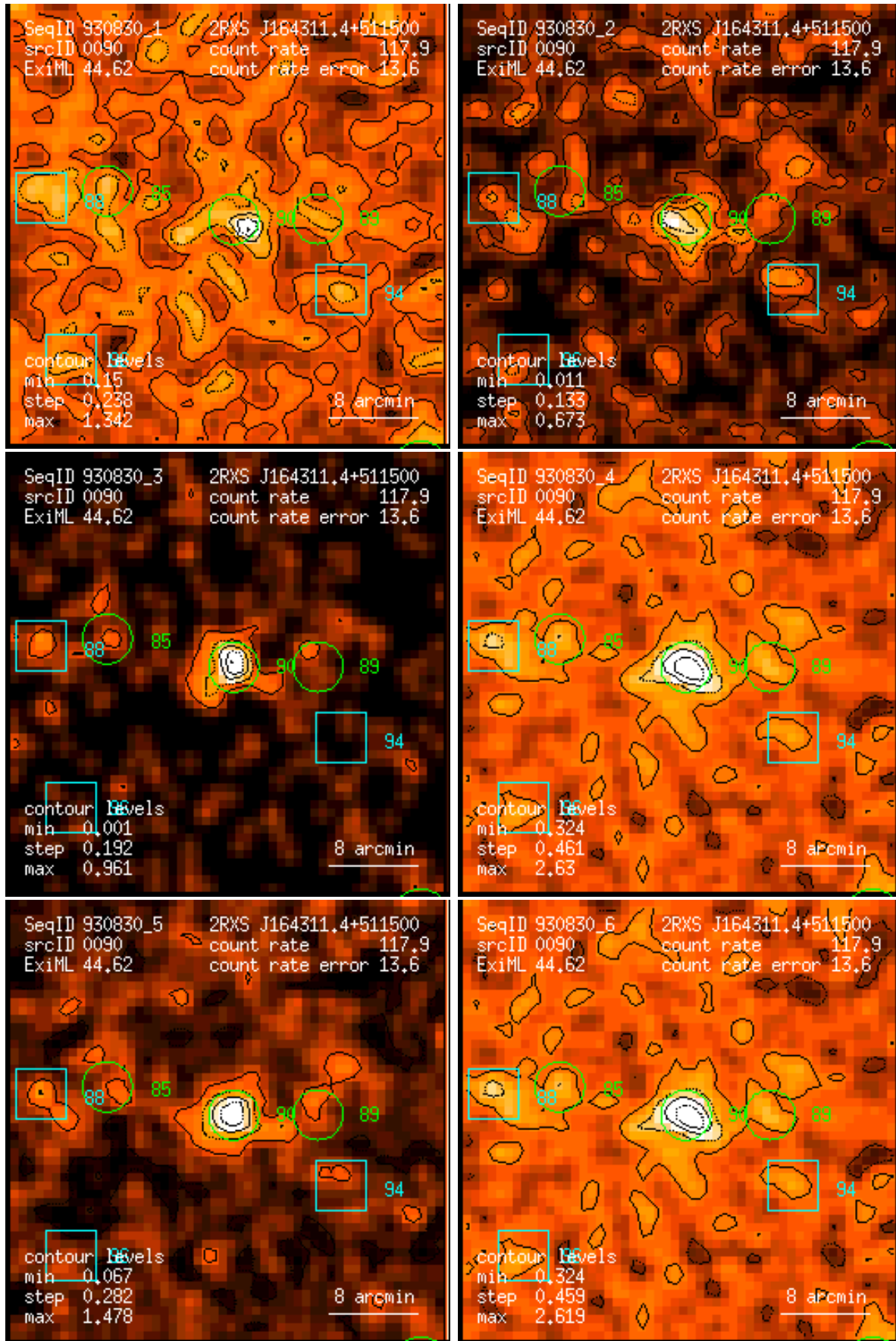
Figure 90: RASS 930830: detection 0090: band rate images, Gaussian filter: (1) PSPC channels 11 – 41, (2) 52 – 90, (3) 91 – 201, (4) 11 – 235, (5) 52 – 201, (6) 11 – 201. Broad band rates in counts/ks. Band rate contour levels in counts/ks/arcmin 2 .
