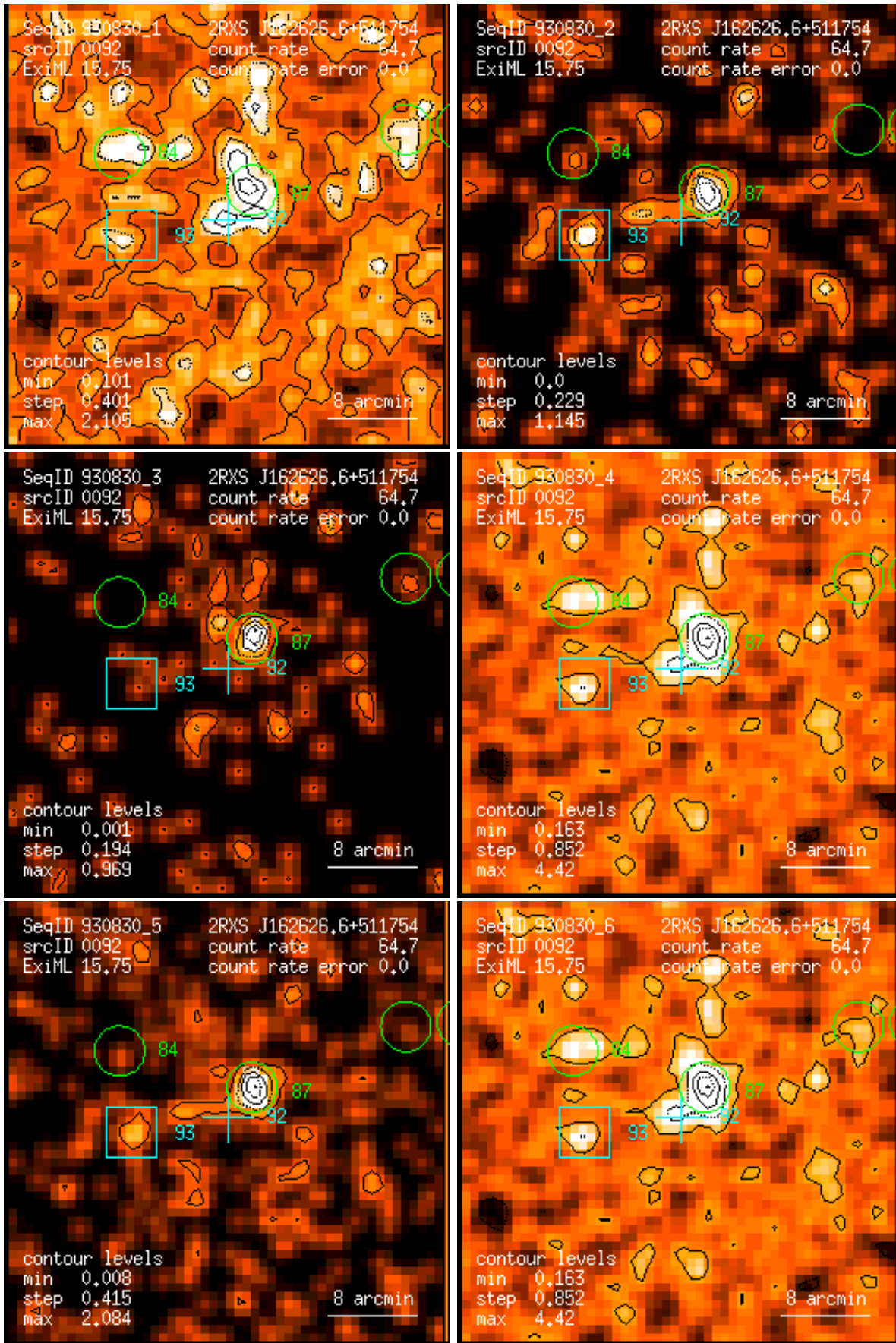
Figure 92: RASS 930830: detection 0092: band rate images, Gaussian filter: (1) PSPC channels 11 – 41, (2) 52 – 90, (3) 91 – 201, (4) 11 – 235, (5) 52 – 201, (6) 11 – 201. Broad band rates in counts/ks. Band rate contour levels in counts/ks/arcmin 2 .
