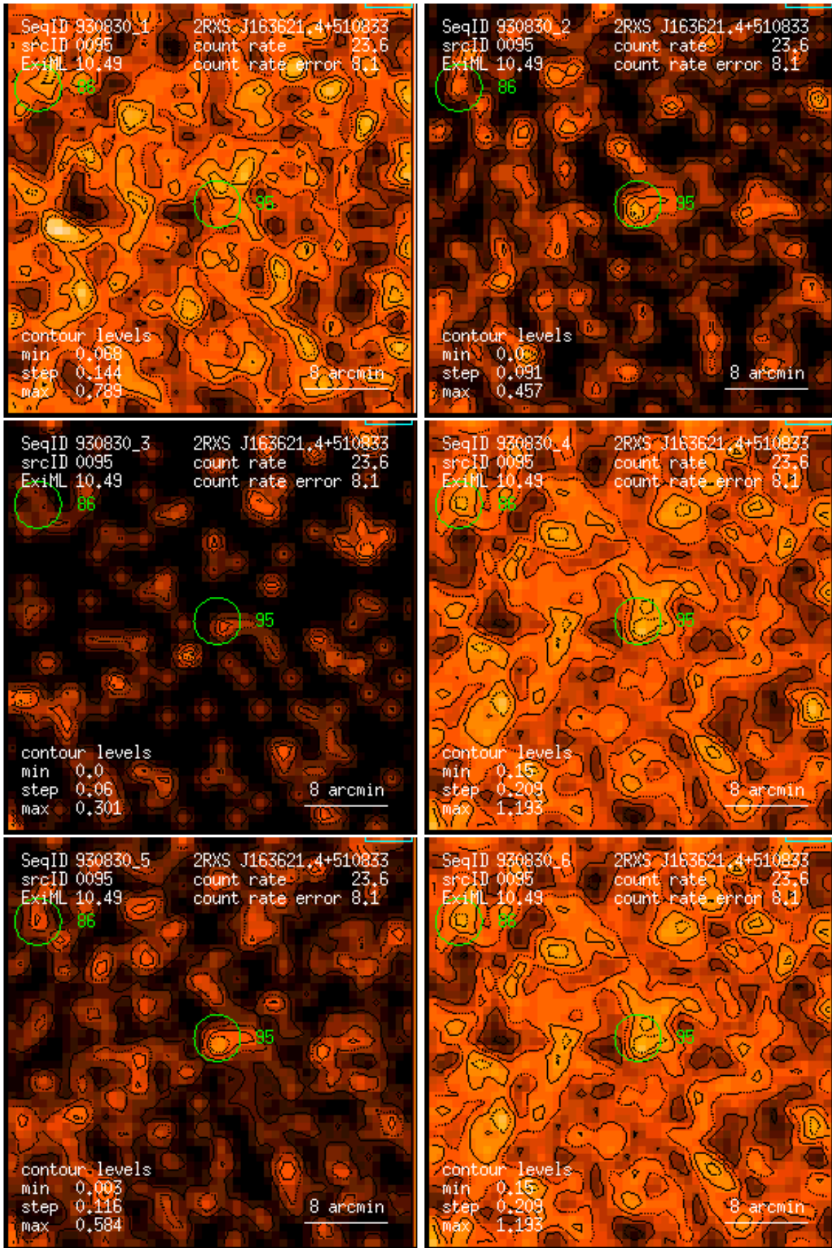
Figure 95: RASS 930830: detection 0095: band rate images, Gaussian filter: (1) PSPC channels 11 – 41, (2) 52 – 90, (3) 91 – 201, (4) 11 – 235, (5) 52 – 201, (6) 11 – 201. Broad band rates in counts/ks. Band rate contour levels in counts/ks/arcmin 2 .
