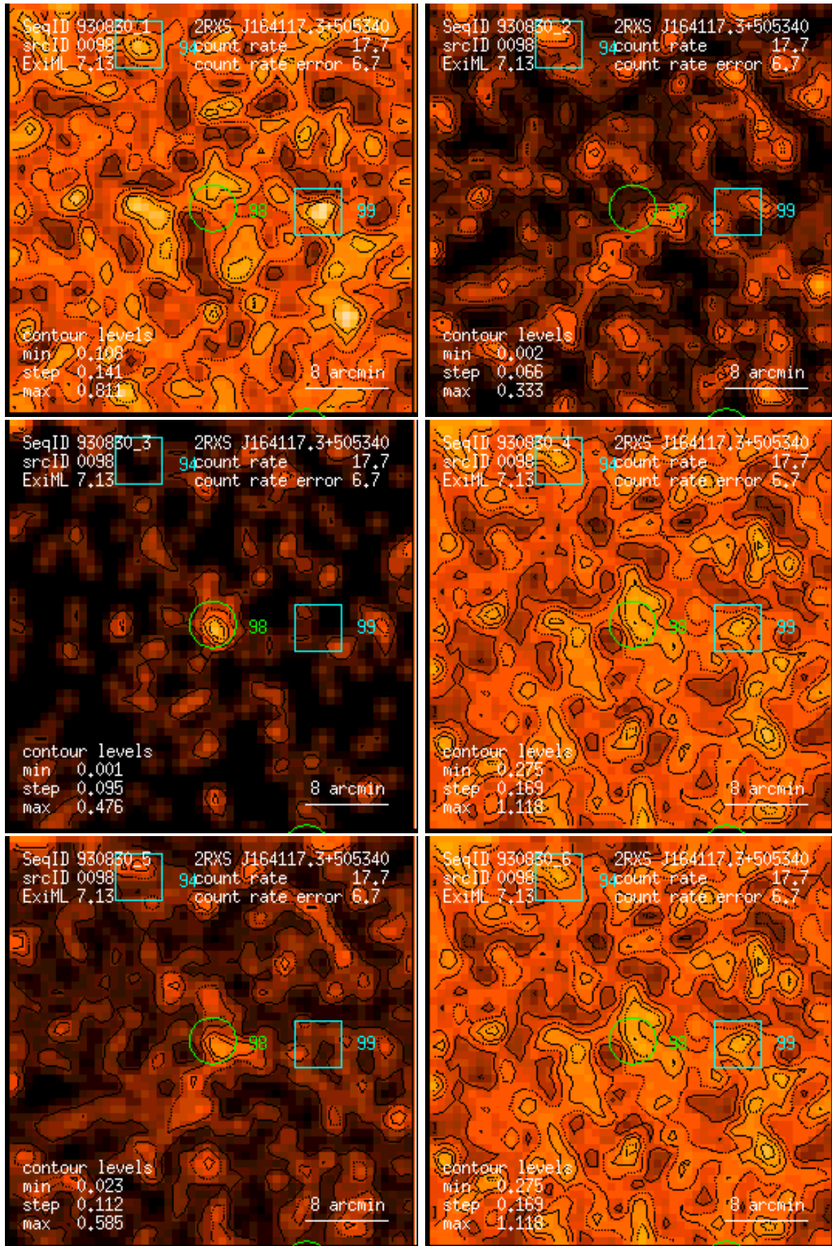
Figure 98: RASS 930830: detection 0098: band rate images, Gaussian filter: (1) PSPC channels 11 – 41, (2) 52 – 90, (3) 91 – 201, (4) 11 – 235, (5) 52 – 201, (6) 11 – 201. Broad band rates in counts/ks. Band rate contour levels in counts/ks/arcmin 2 .
