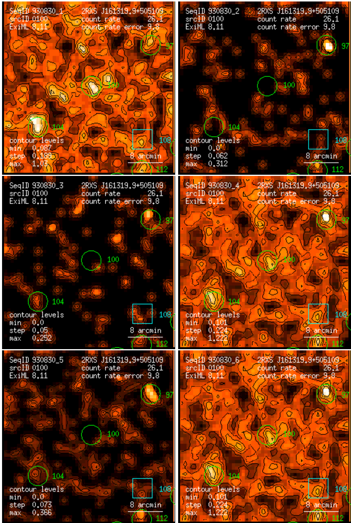
Figure 100: RASS 930830: detection 0100: band rate images, Gaussian filter: (1) PSPC channels 11 – 41, (2) 52 – 90, (3) 91 – 201, (4) 11 – 235, (5) 52 – 201, (6) 11 – 201. Broad band rates in counts/ks. Band rate contour levels in counts/ks/arcmin 2 .
