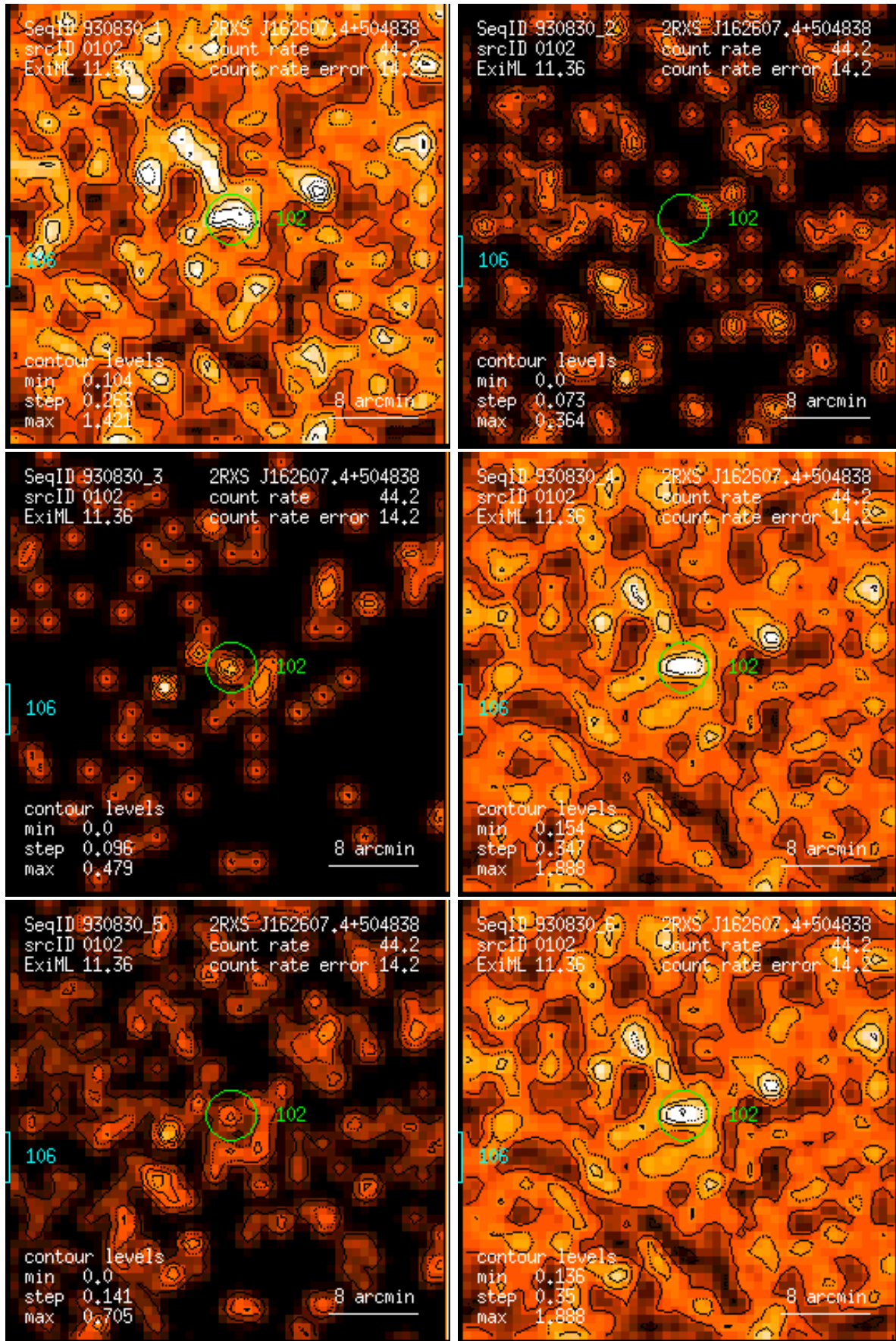
Figure 102: RASS 930830: detection 0102: band rate images, Gaussian filter: (1) PSPC channels 11 – 41, (2) 52 – 90, (3) 91 – 201, (4) 11 – 235, (5) 52 – 201, (6) 11 – 201. Broad band rates in counts/ks. Band rate contour levels in counts/ks/arcmin 2 .
