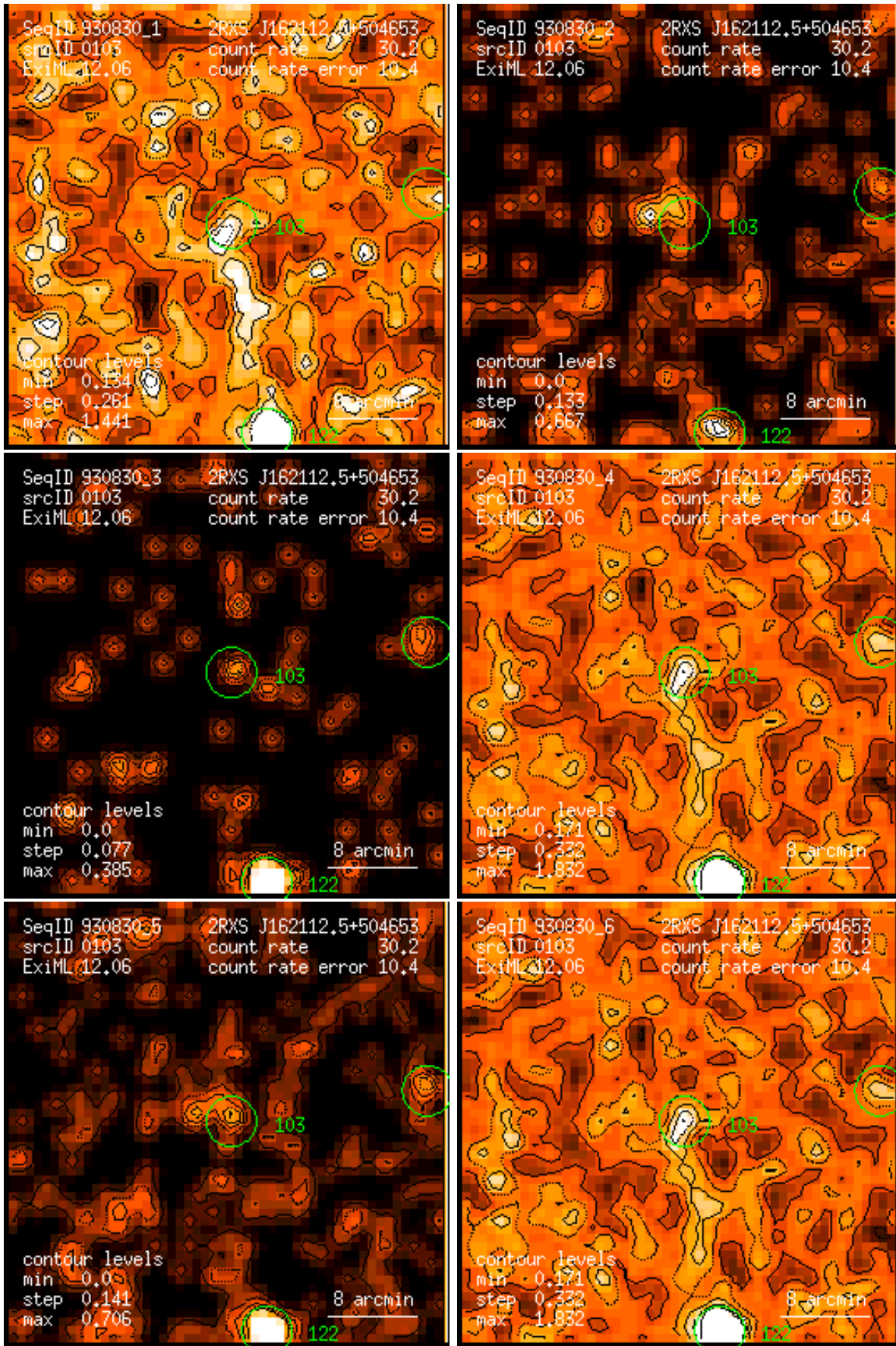
Figure 103: RASS 930830: detection 0103: band rate images, Gaussian filter: (1) PSPC channels 11 – 41, (2) 52 – 90, (3) 91 – 201, (4) 11 – 235, (5) 52 – 201, (6) 11 – 201. Broad band rates in counts/ks. Band rate contour levels in counts/ks/arcmin 2 .
