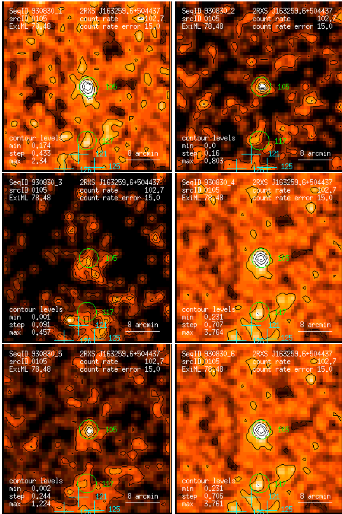
Figure 105: RASS 930830: detection 0105: band rate images, Gaussian filter: (1) PSPC channels 11 – 41, (2) 52 – 90, (3) 91 – 201, (4) 11 – 235, (5) 52 – 201, (6) 11 – 201. Broad band rates in counts/ks. Band rate contour levels in counts/ks/arcmin 2 .
