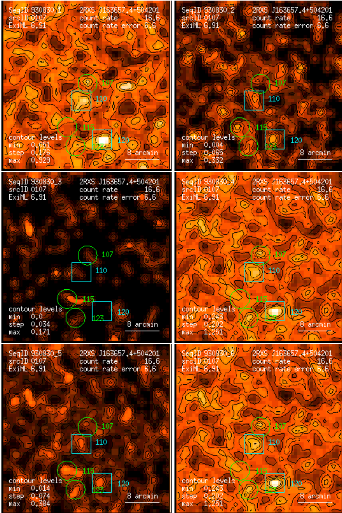
Figure 107: RASS 930830: detection 0107: band rate images, Gaussian filter: (1) PSPC channels 11 – 41, (2) 52 – 90, (3) 91 – 201, (4) 11 – 235, (5) 52 – 201, (6) 11 – 201. Broad band rates in counts/ks. Band rate contour levels in counts/ks/arcmin 2 .
