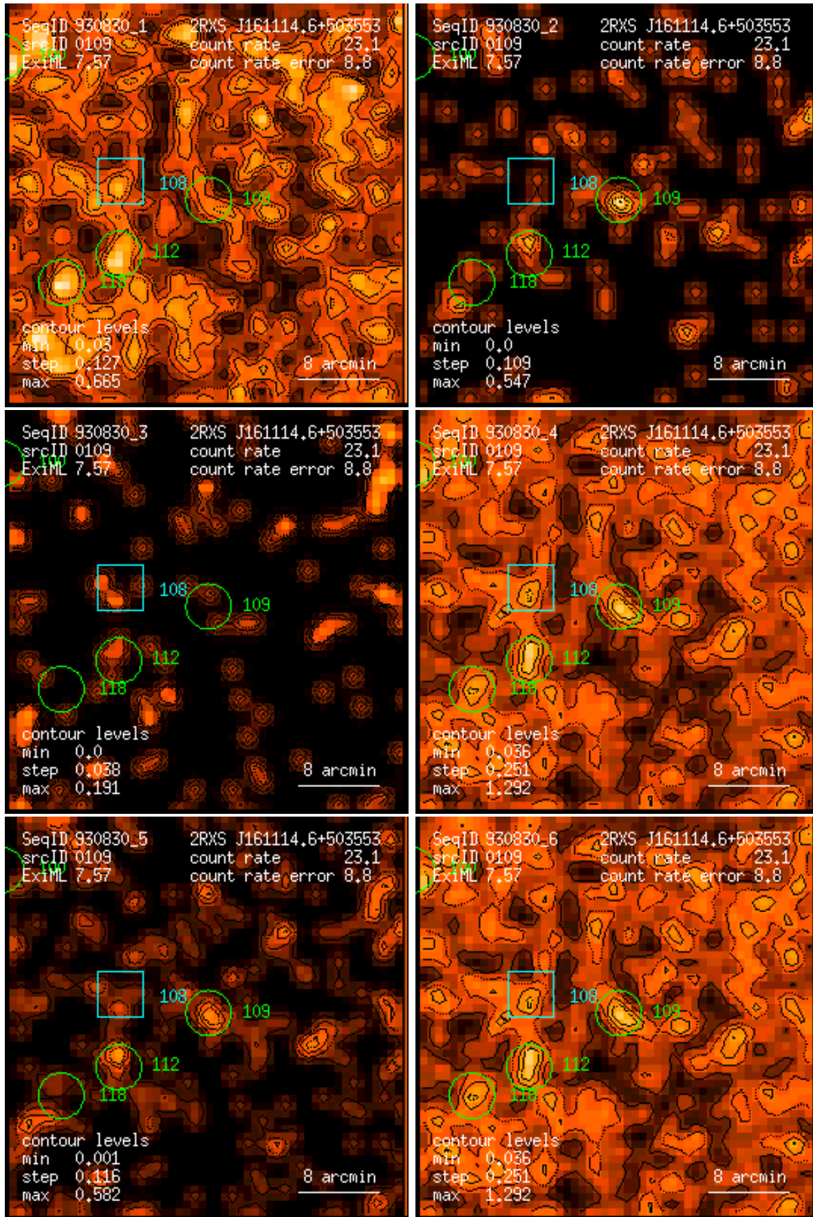
Figure 109: RASS 930830: detection 0109: band rate images, Gaussian filter: (1) PSPC channels 11 – 41, (2) 52 – 90, (3) 91 – 201, (4) 11 – 235, (5) 52 – 201, (6) 11 – 201. Broad band rates in counts/ks. Band rate contour levels in counts/ks/arcmin 2 .
