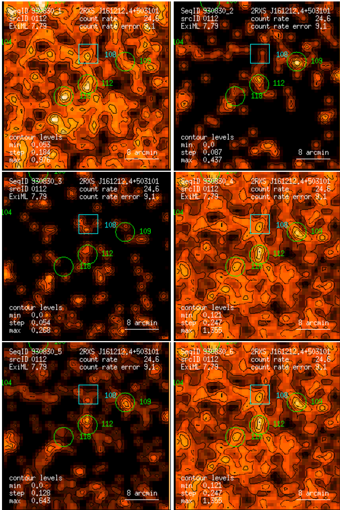
Figure 112: RASS 930830: detection 0112: band rate images, Gaussian filter: (1) PSPC channels 11 – 41, (2) 52 – 90, (3) 91 – 201, (4) 11 – 235, (5) 52 – 201, (6) 11 – 201. Broad band rates in counts/ks. Band rate contour levels in counts/ks/arcmin 2 .
