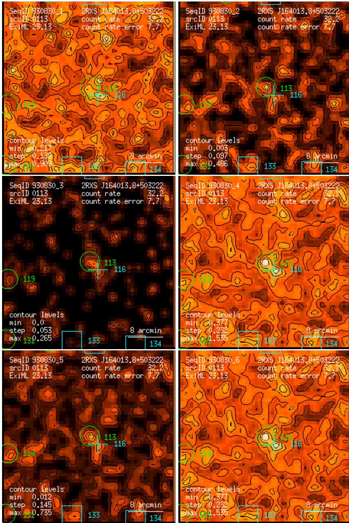
Figure 113: RASS 930830: detection 0113: band rate images, Gaussian filter: (1) PSPC channels 11 – 41, (2) 52 – 90, (3) 91 – 201, (4) 11 – 235, (5) 52 – 201, (6) 11 – 201. Broad band rates in counts/ks. Band rate contour levels in counts/ks/arcmin 2 .
