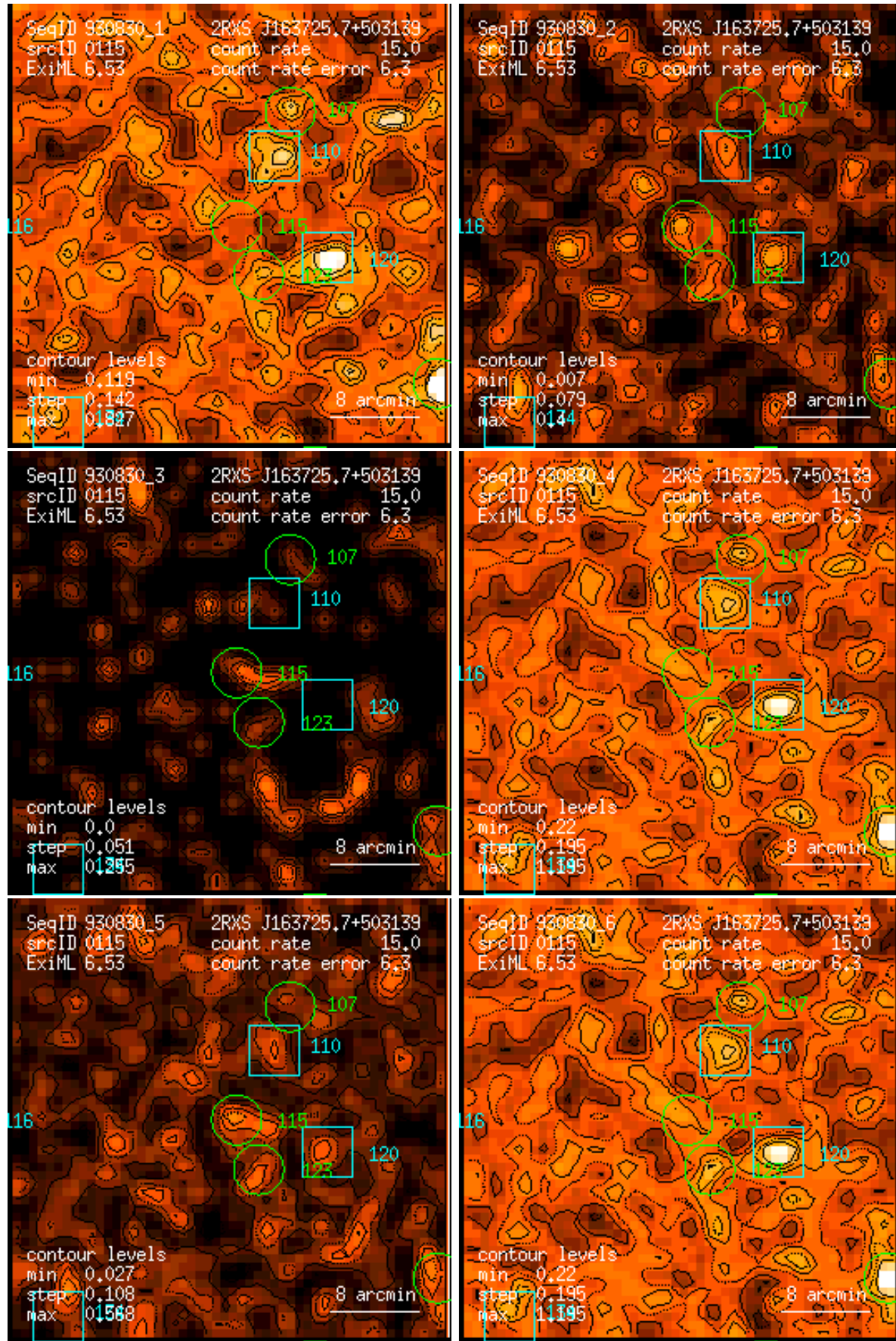
Figure 115: RASS 930830: detection 0115: band rate images, Gaussian filter: (1) PSPC channels 11 – 41, (2) 52 – 90, (3) 91 – 201, (4) 11 – 235, (5) 52 – 201, (6) 11 – 201. Broad band rates in counts/ks. Band rate contour levels in counts/ks/arcmin 2 .
