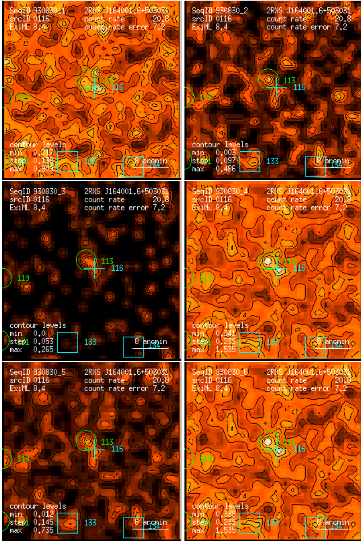
Figure 116: RASS 930830: detection 0116: band rate images, Gaussian filter: (1) PSPC channels 11 – 41, (2) 52 – 90, (3) 91 – 201, (4) 11 – 235, (5) 52 – 201, (6) 11 – 201. Broad band rates in counts/ks. Band rate contour levels in counts/ks/arcmin 2 .
