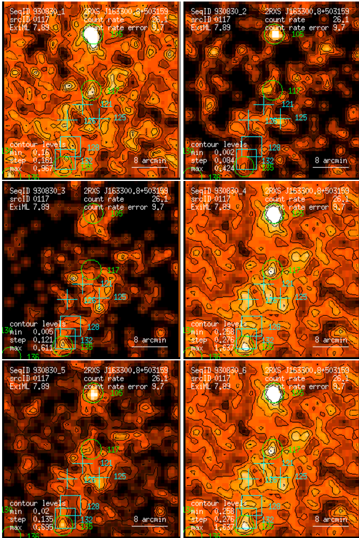
Figure 117: RASS 930830: detection 0117: band rate images, Gaussian filter: (1) PSPC channels 11 – 41, (2) 52 – 90, (3) 91 – 201, (4) 11 – 235, (5) 52 – 201, (6) 11 – 201. Broad band rates in counts/ks. Band rate contour levels in counts/ks/arcmin 2 .
