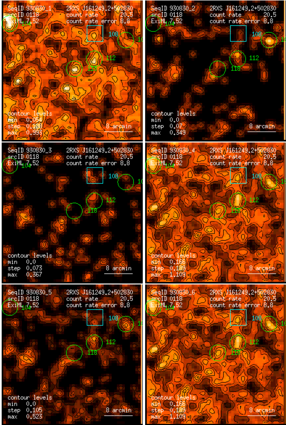
Figure 118: RASS 930830: detection 0118: band rate images, Gaussian filter: (1) PSPC channels 11 – 41, (2) 52 – 90, (3) 91 – 201, (4) 11 – 235, (5) 52 – 201, (6) 11 – 201. Broad band rates in counts/ks. Band rate contour levels in counts/ks/arcmin 2 .
