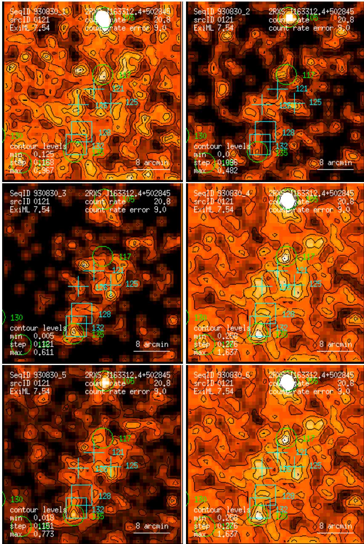
Figure 121: RASS 930830: detection 0121: band rate images, Gaussian filter: (1) PSPC channels 11 – 41, (2) 52 – 90, (3) 91 – 201, (4) 11 – 235, (5) 52 – 201, (6) 11 – 201. Broad band rates in counts/ks. Band rate contour levels in counts/ks/arcmin 2 .
