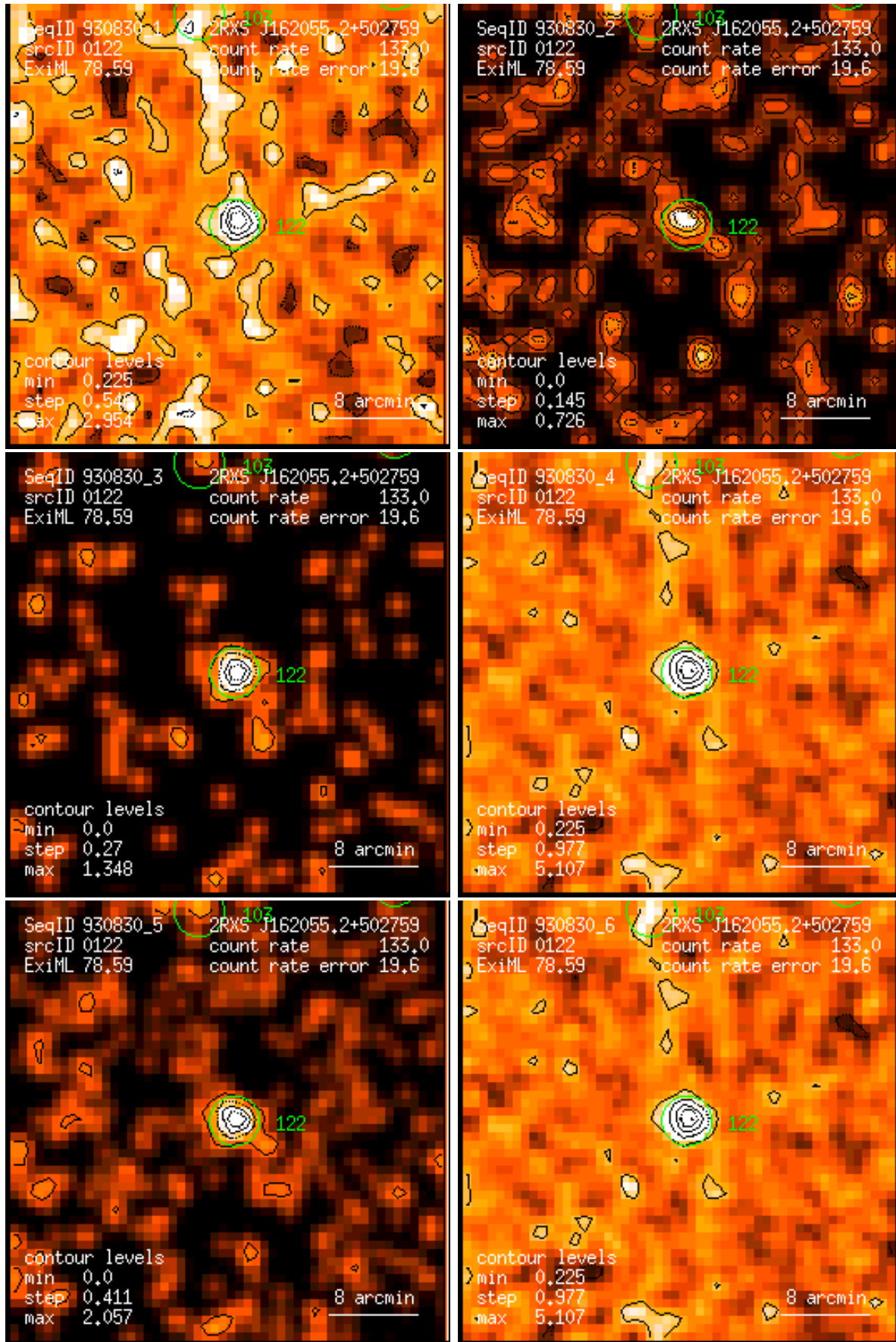
Figure 122: RASS 930830: detection 0122: band rate images, Gaussian filter: (1) PSPC channels 11 – 41, (2) 52 – 90, (3) 91 – 201, (4) 11 – 235, (5) 52 – 201, (6) 11 – 201. Broad band rates in counts/ks. Band rate contour levels in counts/ks/arcmin 2 .
