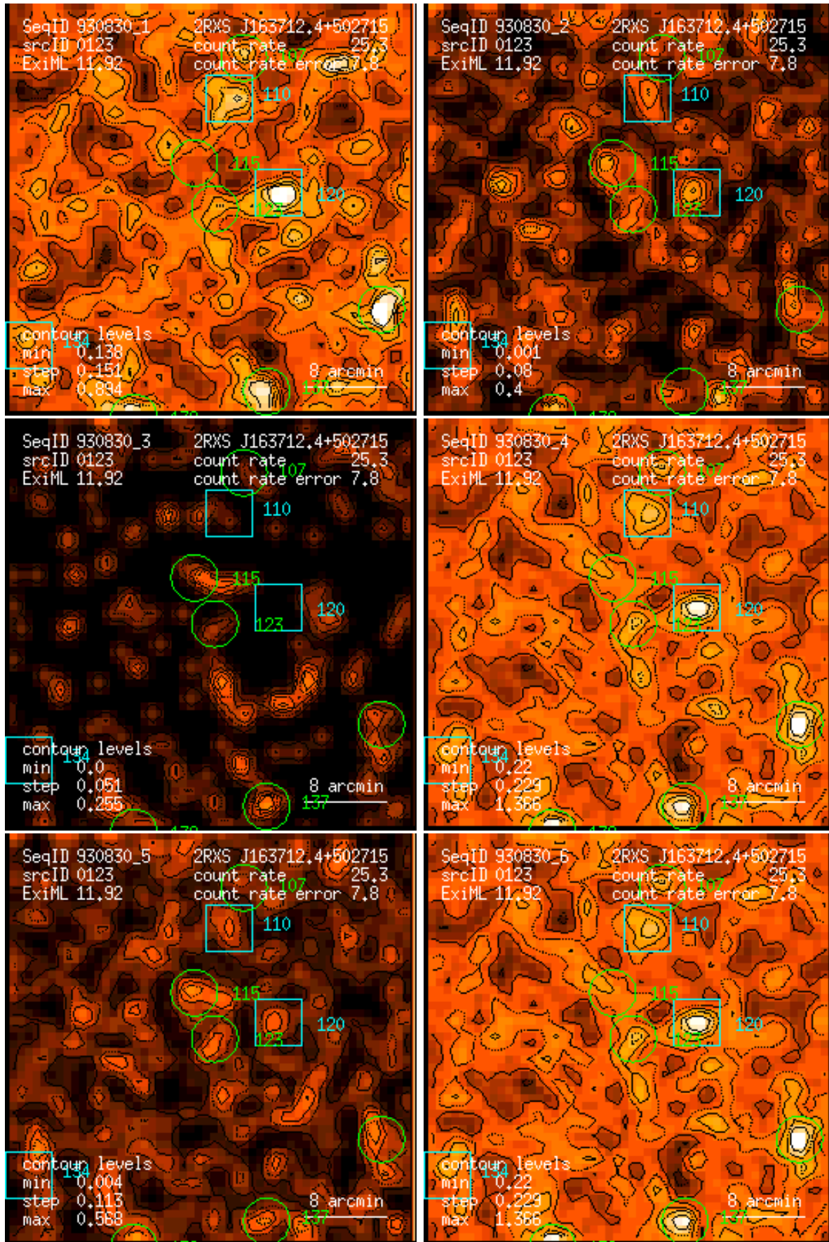
Figure 123: RASS 930830: detection 0123: band rate images, Gaussian filter: (1) PSPC channels 11 – 41, (2) 52 – 90, (3) 91 – 201, (4) 11 – 235, (5) 52 – 201, (6) 11 – 201. Broad band rates in counts/ks. Band rate contour levels in counts/ks/arcmin 2 .
