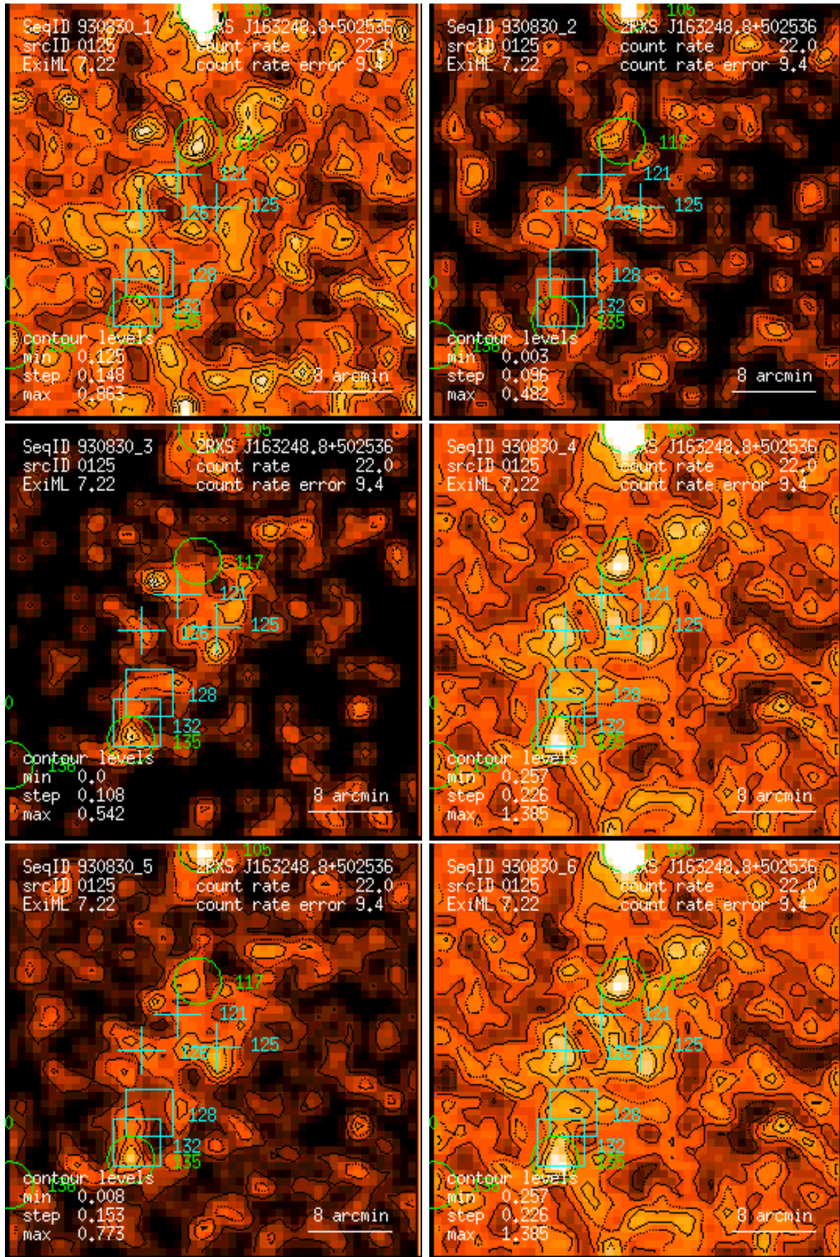
Figure 125: RASS 930830: detection 0125: band rate images, Gaussian filter: (1) PSPC channels 11 – 41, (2) 52 – 90, (3) 91 – 201, (4) 11 – 235, (5) 52 – 201, (6) 11 – 201. Broad band rates in counts/ks. Band rate contour levels in counts/ks/arcmin 2 .
