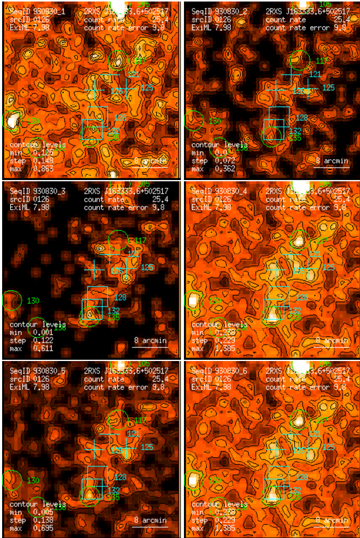
Figure 126: RASS 930830: detection 0126: band rate images, Gaussian filter: (1) PSPC channels 11 – 41, (2) 52 – 90, (3) 91 – 201, (4) 11 – 235, (5) 52 – 201, (6) 11 – 201. Broad band rates in counts/ks. Band rate contour levels in counts/ks/arcmin 2 .
