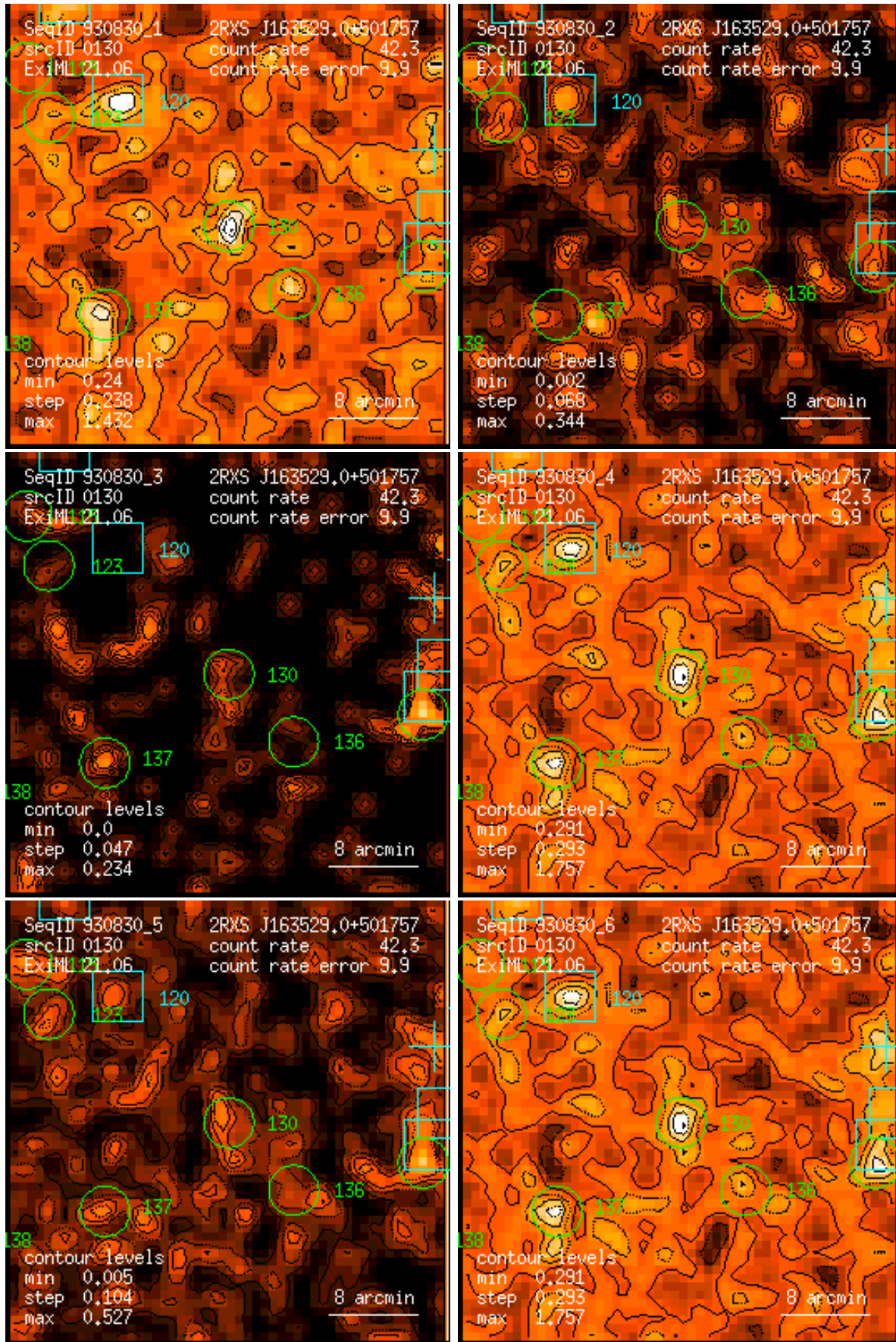
Figure 130: RASS 930830: detection 0130: band rate images, Gaussian filter: (1) PSPC channels 11 – 41, (2) 52 – 90, (3) 91 – 201, (4) 11 – 235, (5) 52 – 201, (6) 11 – 201. Broad band rates in counts/ks. Band rate contour levels in counts/ks/arcmin 2 .
