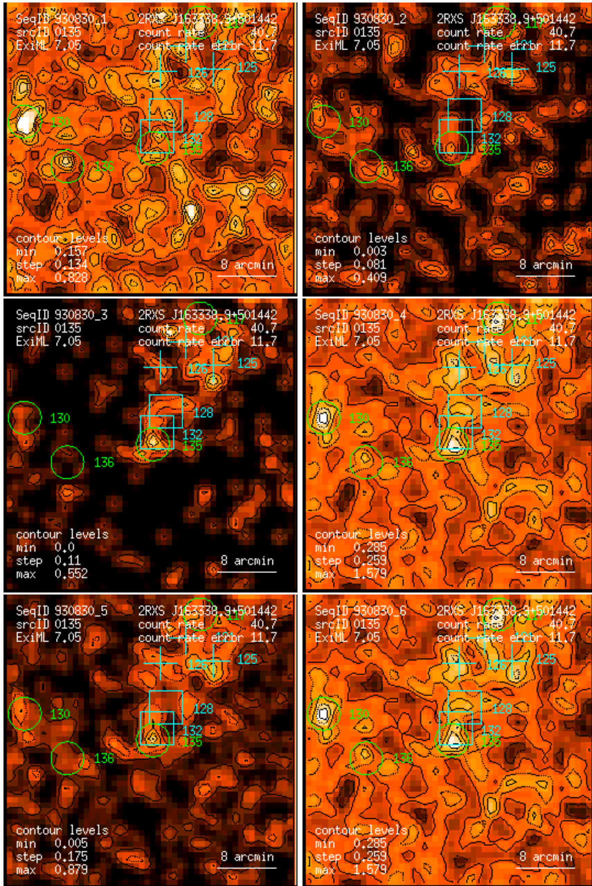
Figure 135: RASS 930830: detection 0135: band rate images, Gaussian filter: (1) PSPC channels 11 – 41, (2) 52 – 90, (3) 91 – 201, (4) 11 – 235, (5) 52 – 201, (6) 11 – 201. Broad band rates in counts/ks. Band rate contour levels in counts/ks/arcmin 2 .
