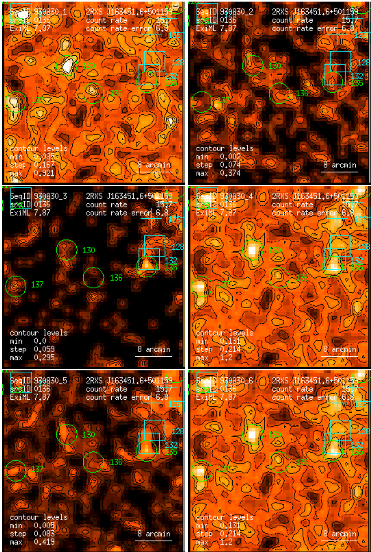
Figure 136: RASS 930830: detection 0136: band rate images, Gaussian filter: (1) PSPC channels 11 – 41, (2) 52 – 90, (3) 91 – 201, (4) 11 – 235, (5) 52 – 201, (6) 11 – 201. Broad band rates in counts/ks. Band rate contour levels in counts/ks/arcmin 2 .
