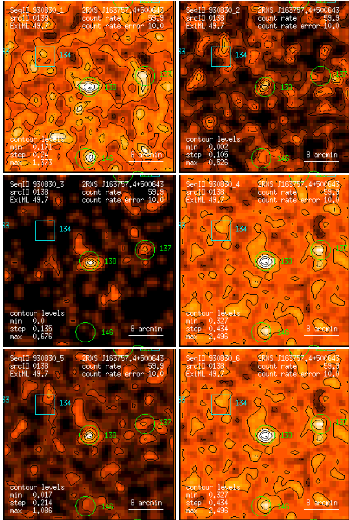
Figure 138: RASS 930830: detection 0138: band rate images, Gaussian filter: (1) PSPC channels 11 – 41, (2) 52 – 90, (3) 91 – 201, (4) 11 – 235, (5) 52 – 201, (6) 11 – 201. Broad band rates in counts/ks. Band rate contour levels in counts/ks/arcmin 2 .
