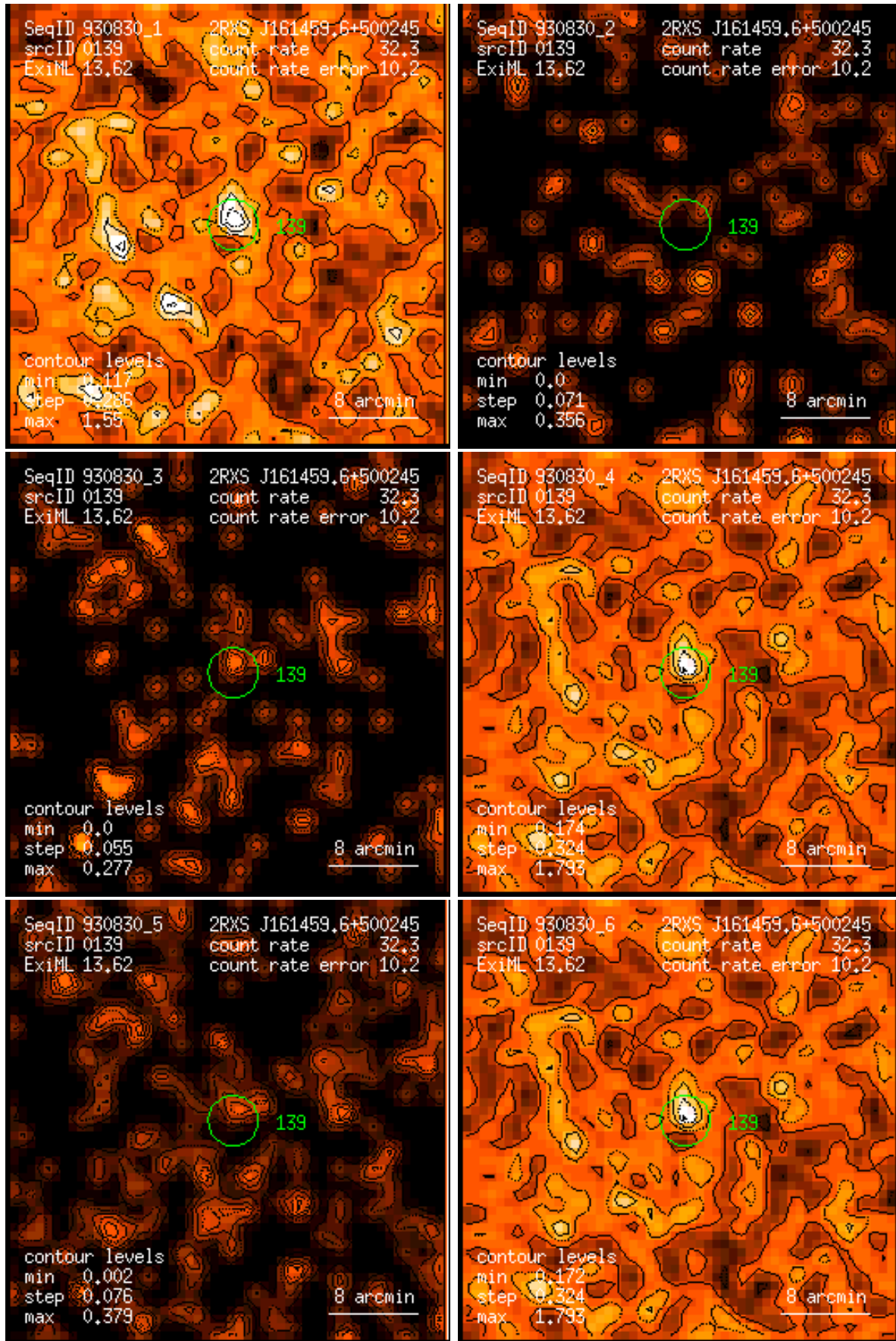
Figure 139: RASS 930830: detection 0139: band rate images, Gaussian filter: (1) PSPC channels 11 – 41, (2) 52 – 90, (3) 91 – 201, (4) 11 – 235, (5) 52 – 201, (6) 11 – 201. Broad band rates in counts/ks. Band rate contour levels in counts/ks/arcmin 2 .
