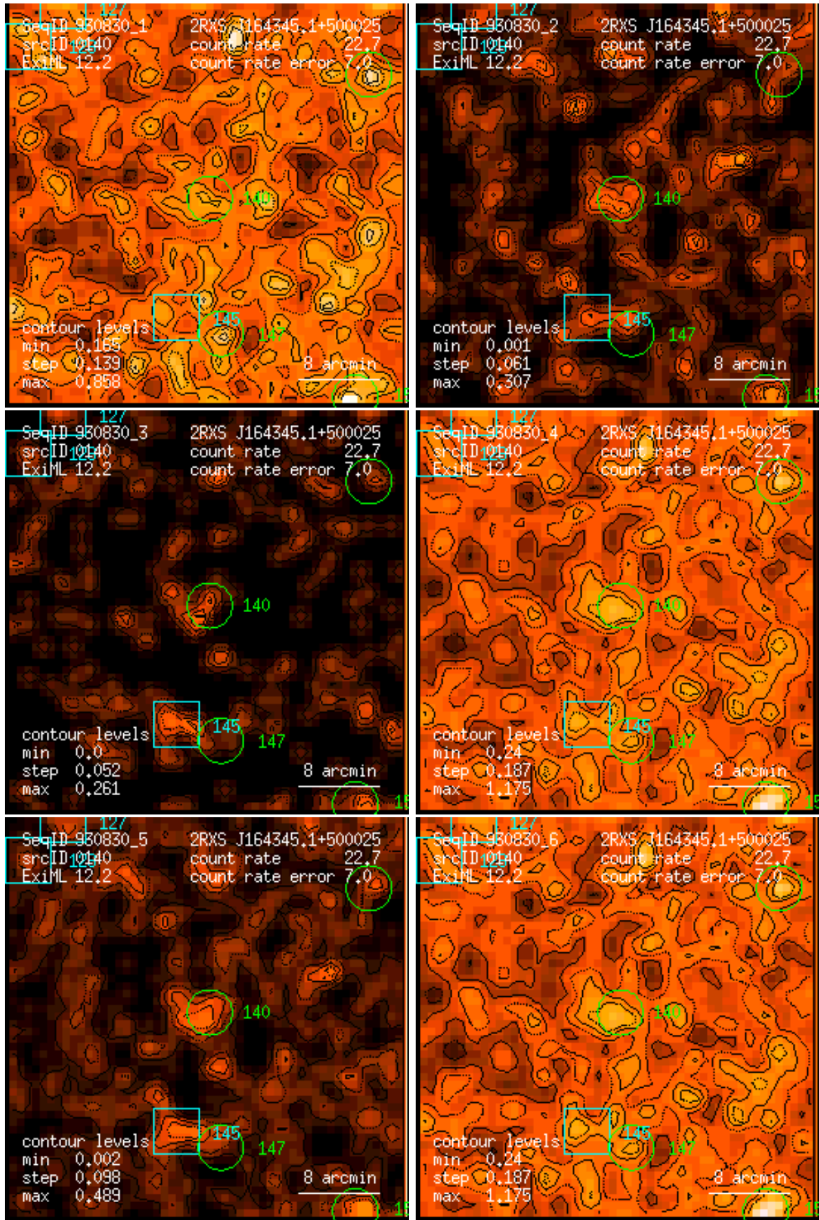
Figure 140: RASS 930830: detection 0140: band rate images, Gaussian filter: (1) PSPC channels 11 – 41, (2) 52 – 90, (3) 91 – 201, (4) 11 – 235, (5) 52 – 201, (6) 11 – 201. Broad band rates in counts/ks. Band rate contour levels in counts/ks/arcmin 2 .
