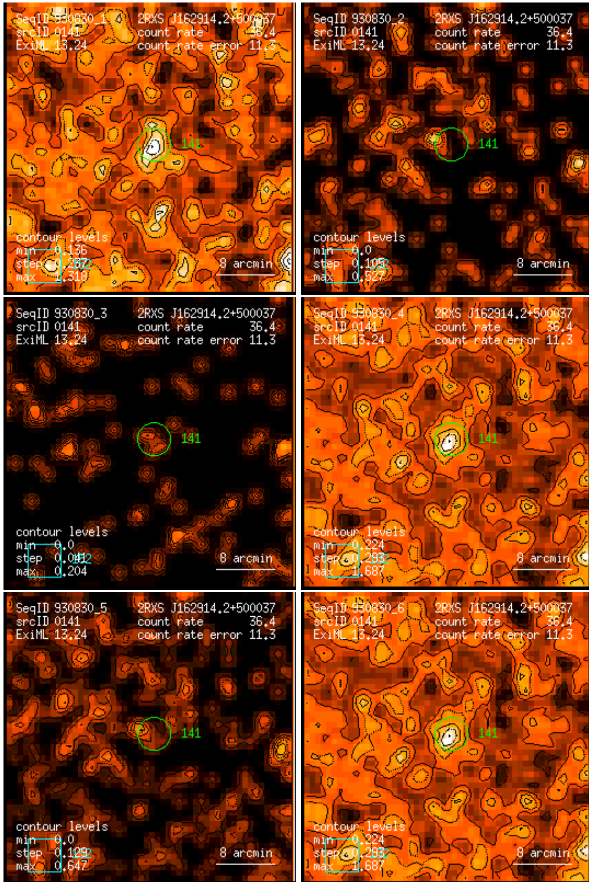
Figure 141: RASS 930830: detection 0141: band rate images, Gaussian filter: (1) PSPC channels 11 – 41, (2) 52 – 90, (3) 91 – 201, (4) 11 – 235, (5) 52 – 201, (6) 11 – 201. Broad band rates in counts/ks. Band rate contour levels in counts/ks/arcmin 2 .
