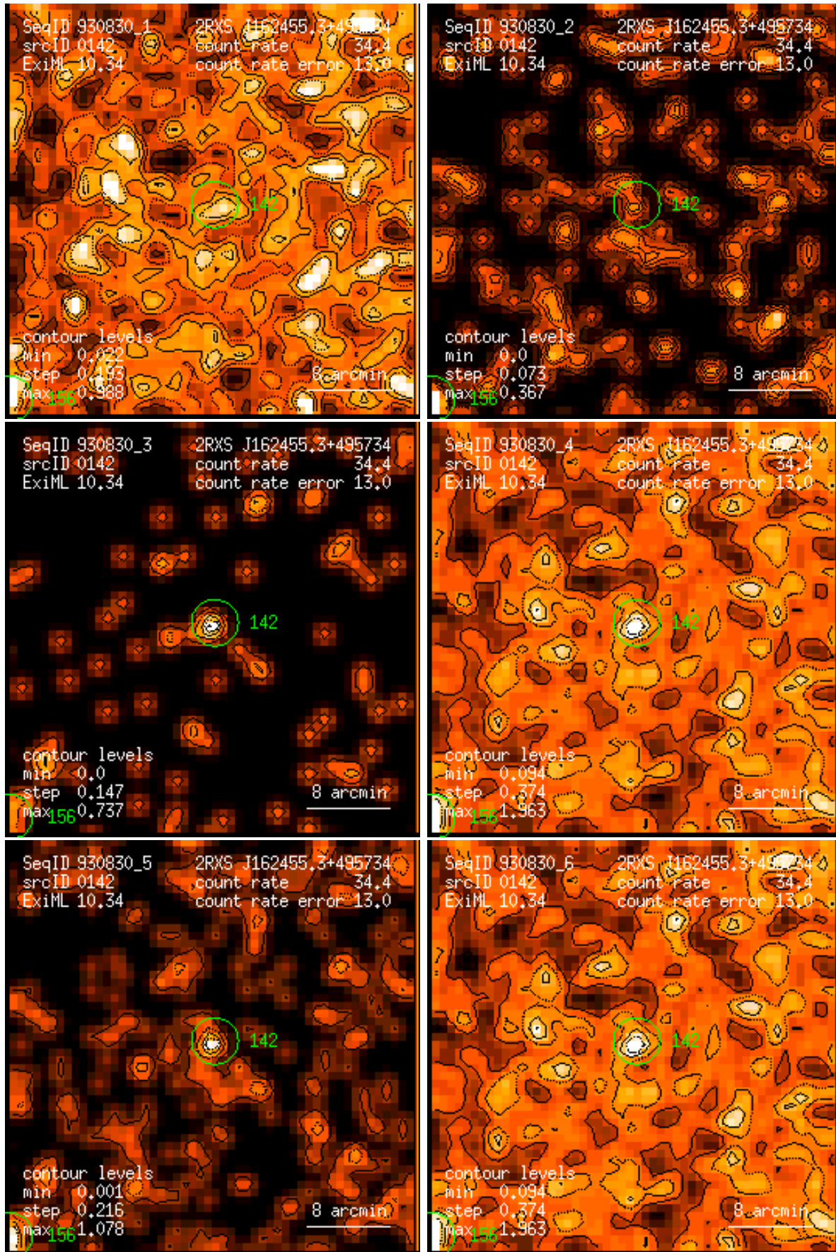
Figure 142: RASS 930830: detection 0142: band rate images, Gaussian filter: (1) PSPC channels 11 – 41, (2) 52 – 90, (3) 91 – 201, (4) 11 – 235, (5) 52 – 201, (6) 11 – 201. Broad band rates in counts/ks. Band rate contour levels in counts/ks/arcmin 2 .
