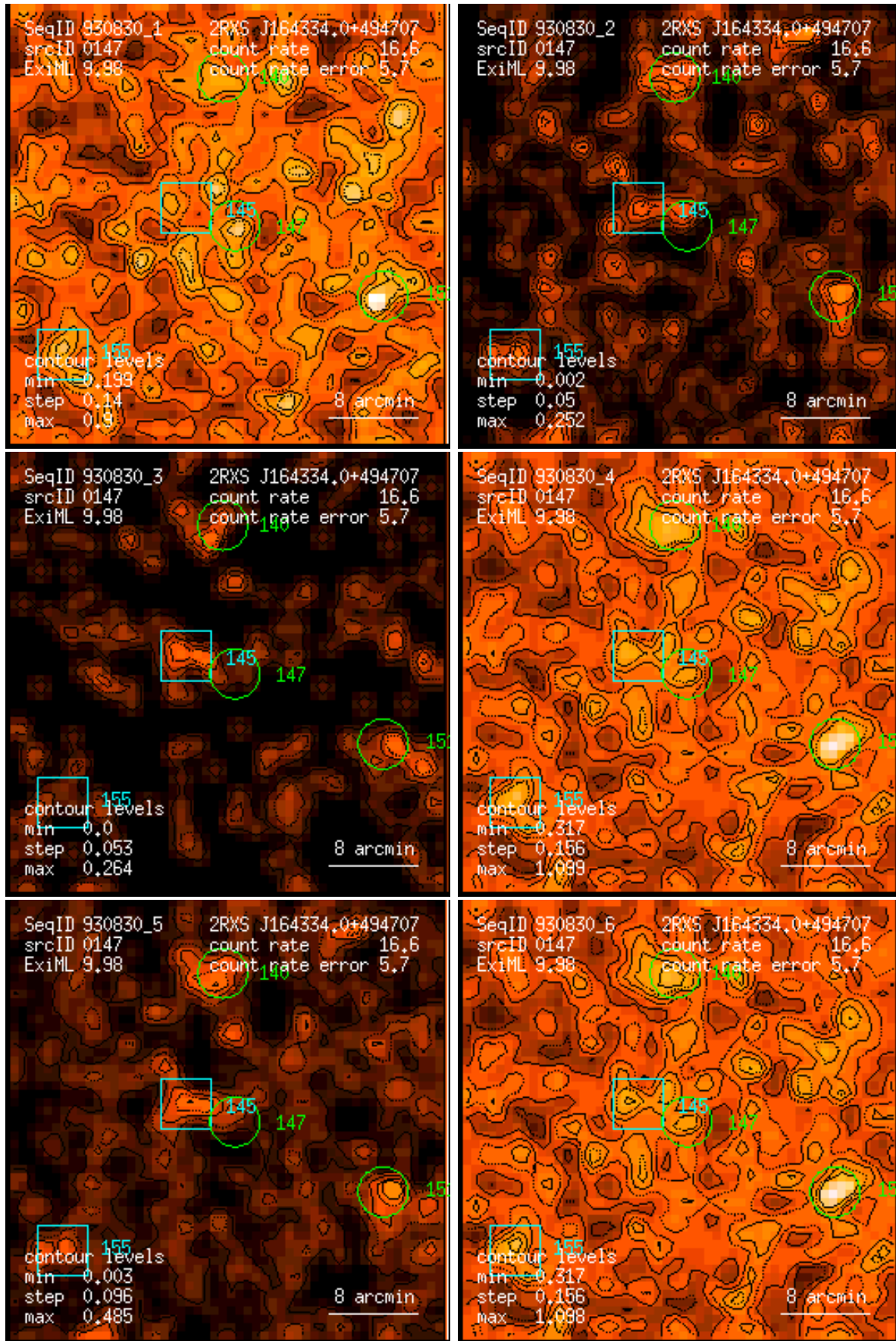
Figure 147: RASS 930830: detection 0147: band rate images, Gaussian filter: (1) PSPC channels 11 – 41, (2) 52 – 90, (3) 91 – 201, (4) 11 – 235, (5) 52 – 201, (6) 11 – 201. Broad band rates in counts/ks. Band rate contour levels in counts/ks/arcmin 2 .
