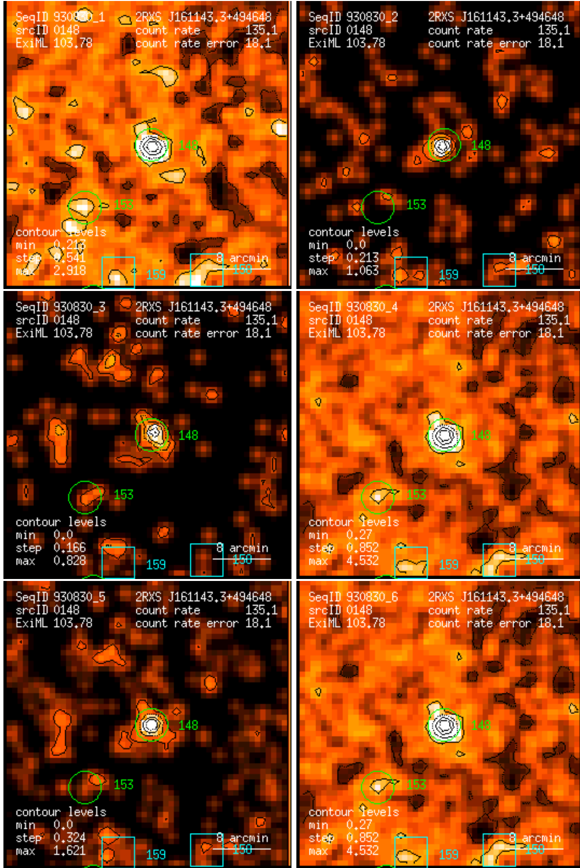
Figure 148: RASS 930830: detection 0148: band rate images, Gaussian filter: (1) PSPC channels 11 – 41, (2) 52 – 90, (3) 91 – 201, (4) 11 – 235, (5) 52 – 201, (6) 11 – 201. Broad band rates in counts/ks. Band rate contour levels in counts/ks/arcmin 2 .
