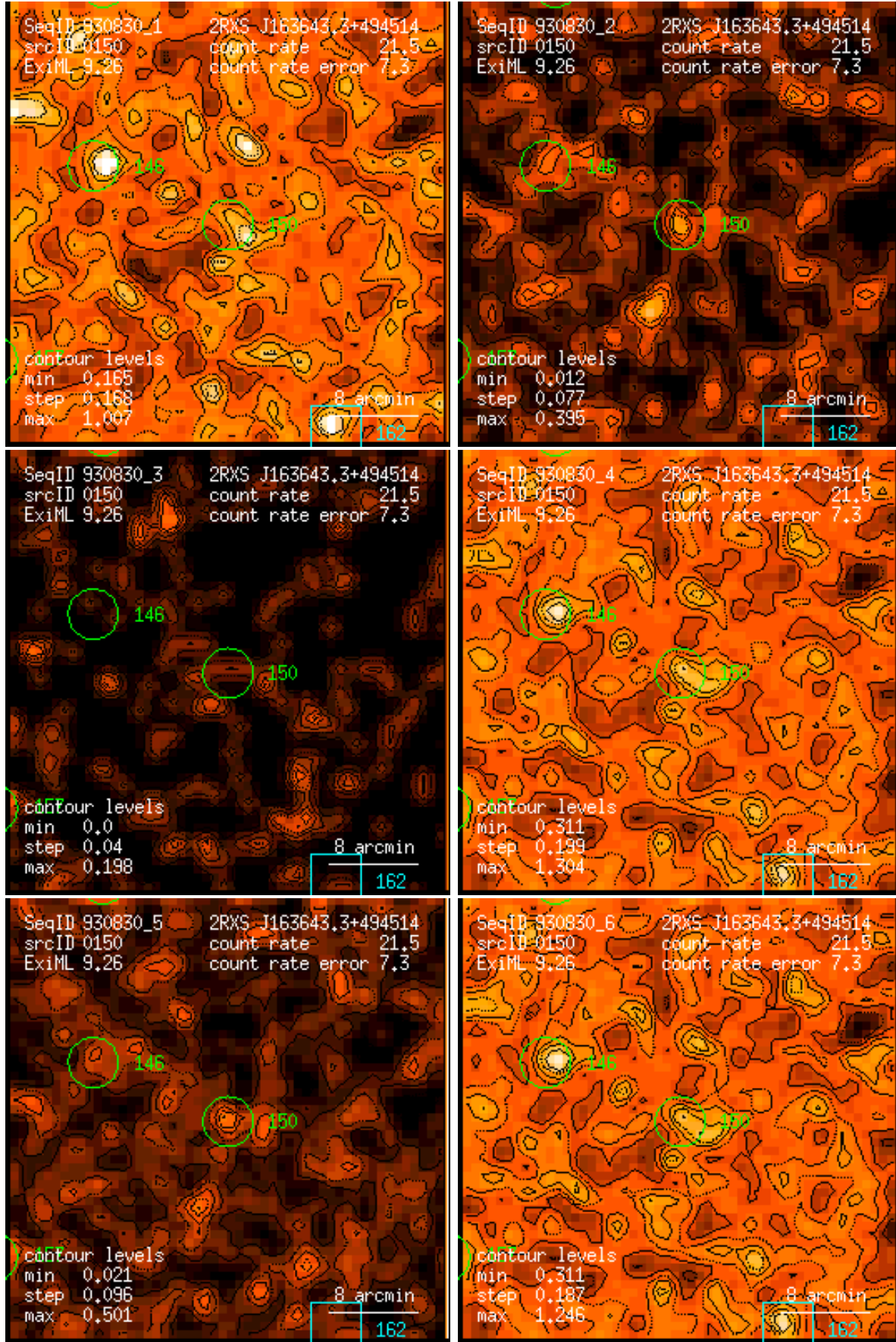
Figure 150: RASS 930830: detection 0150: band rate images, Gaussian filter: (1) PSPC channels 11 – 41, (2) 52 – 90, (3) 91 – 201, (4) 11 – 235, (5) 52 – 201, (6) 11 – 201. Broad band rates in counts/ks. Band rate contour levels in counts/ks/arcmin 2 .
