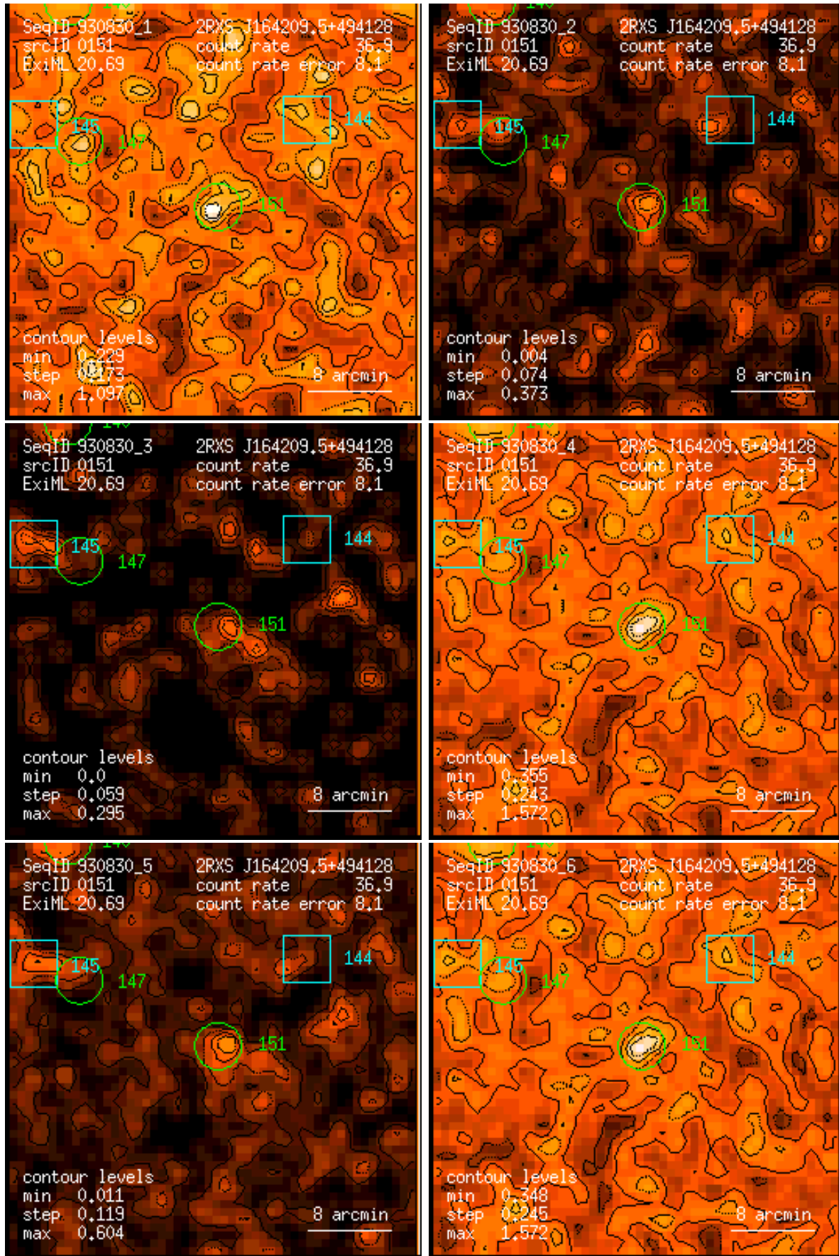
Figure 151: RASS 930830: detection 0151: band rate images, Gaussian filter: (1) PSPC channels 11 – 41, (2) 52 – 90, (3) 91 – 201, (4) 11 – 235, (5) 52 – 201, (6) 11 – 201. Broad band rates in counts/ks. Band rate contour levels in counts/ks/arcmin 2 .
