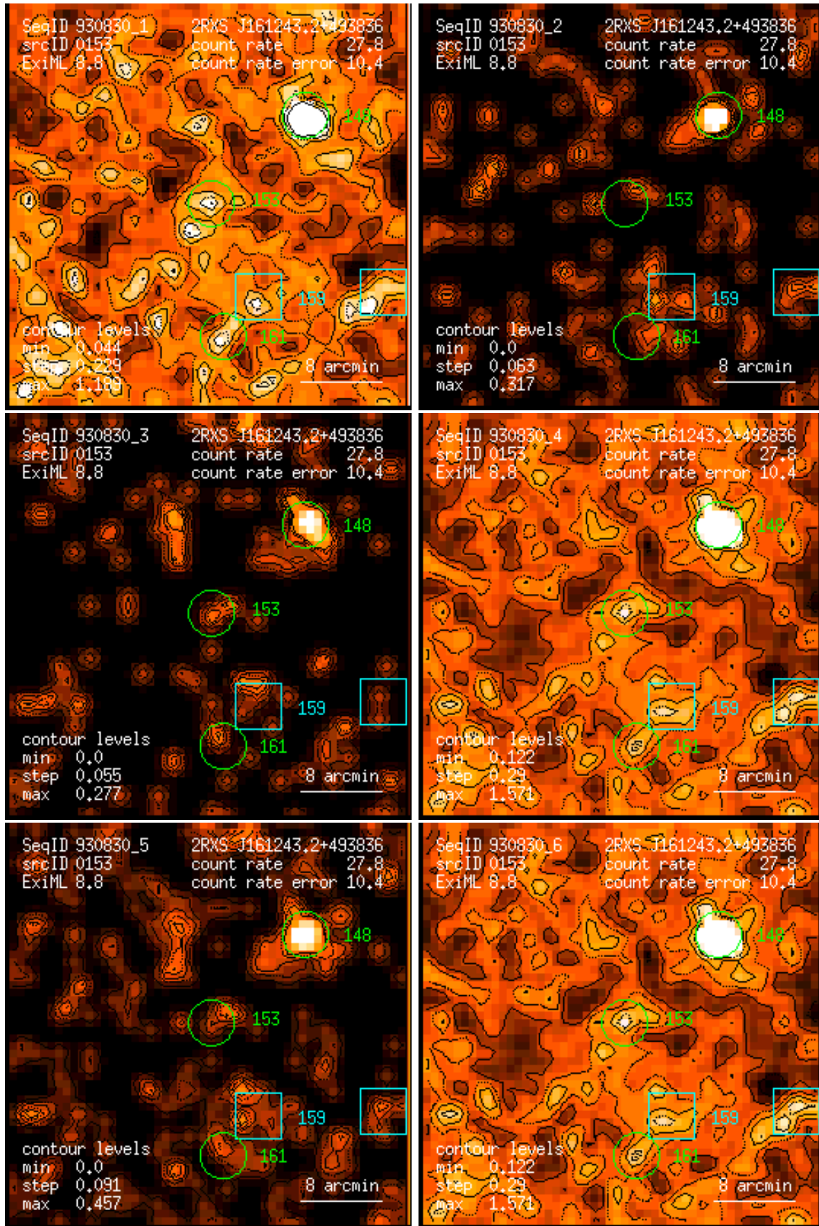
Figure 153: RASS 930830: detection 0153: band rate images, Gaussian filter: (1) PSPC channels 11 – 41, (2) 52 – 90, (3) 91 – 201, (4) 11 – 235, (5) 52 – 201, (6) 11 – 201. Broad band rates in counts/ks. Band rate contour levels in counts/ks/arcmin 2 .
