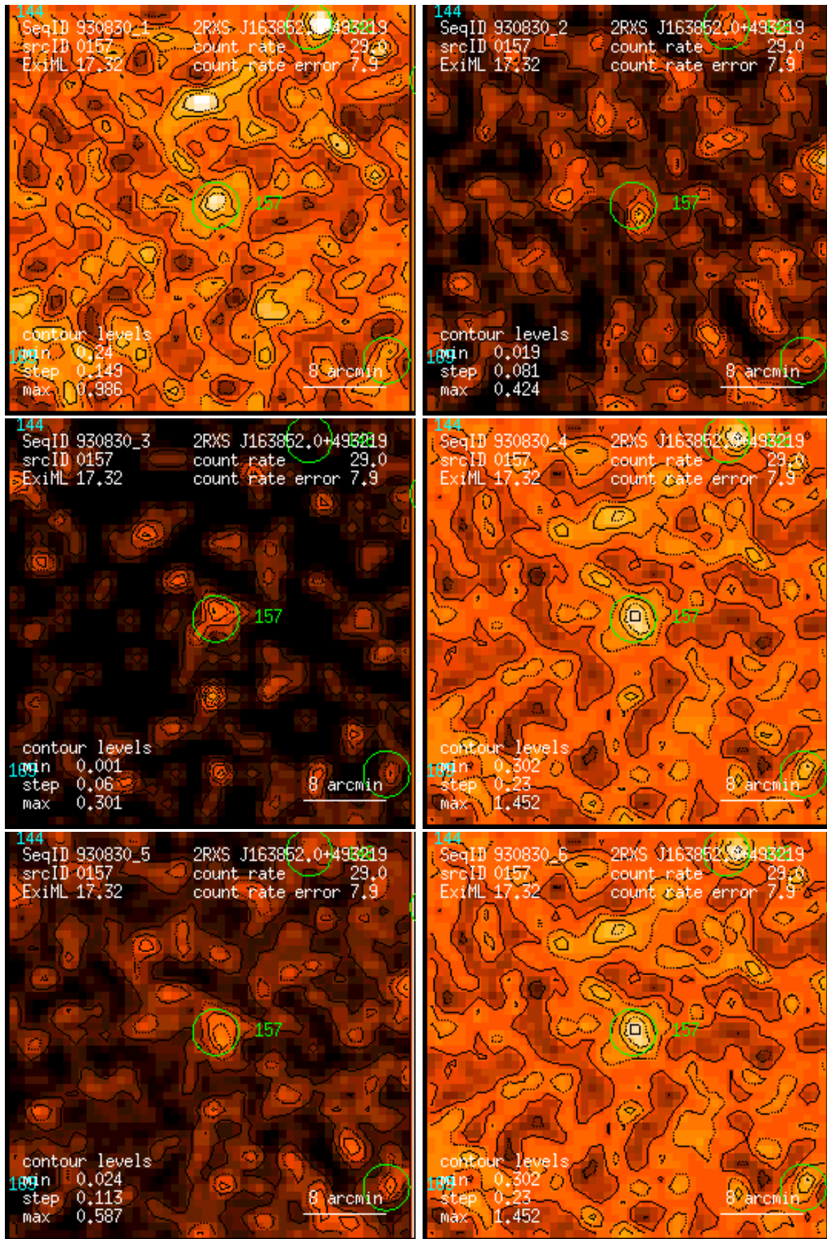
Figure 157: RASS 930830: detection 0157: band rate images, Gaussian filter: (1) PSPC channels 11 – 41, (2) 52 – 90, (3) 91 – 201, (4) 11 – 235, (5) 52 – 201, (6) 11 – 201. Broad band rates in counts/ks. Band rate contour levels in counts/ks/arcmin 2 .
